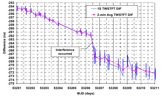
Figure 10. Time step in UTC(NIST) – UTC(PTB) TWSTFT difference due to changes on the satellite transponder (interference, load?).
