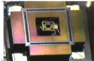
Figure 1: Bonded die of bottom two wafers. The released proof-mass in the center is held by two sets of springs in each corner.
