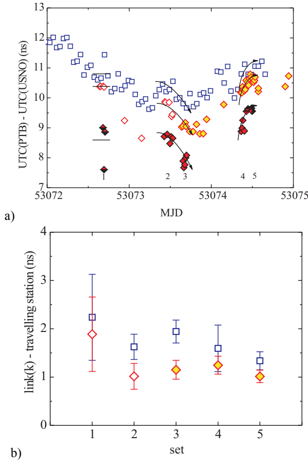
Figure 3. March 2004 results: a) Comparison of the time scales UTC(USNO) and UTC(PTB) using three TWSTFT links during the calibration campaign of March 2004: Ku-band (blue squares), X-band (open red diamonds), and TS (full symbols). Here we distinguish between sets 2 to 4, when the TS standard configuration was used, and sets 1 and 5 when test measurements were carried out using a different reference frequency (set 1), cabling, and modem (set 5). b) Double-differences [UTC(PTB) - UTC(USNO)]_{Ku\text{-band}} - [UTC(PTB) - UTC(USNO)]_{TS} (blue squares) and [UTC(PTB) - UTC(USNO)]_{X\text{-band}} - [UTC(PTB) - UTC(USNO)]_{TS} (red diamonds). The yellow fill indicates that a new LNA in the receiving path of PTB's X-band station was installed.
