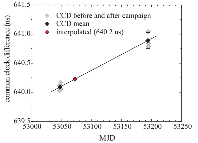
Figure 2. Initial (February 13) and closure (July 8) measurements for the Mar'04 calibration at USNO. Gray diamonds represent single measurements, and black diamonds and error bars represent the mean and standard deviation, respectively. Interpolation of both results (red diamond) provides the common clock difference between permanent and the travelling station (TS) of USNO for the epoch of the TS operation at PTB.
