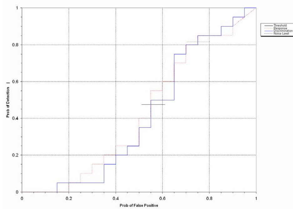
Figure 2. EM61 MKII/towed array blind grid probability of detection for response and discrimination stages versus their respective probability of false positive over all ordnance categories combined.
