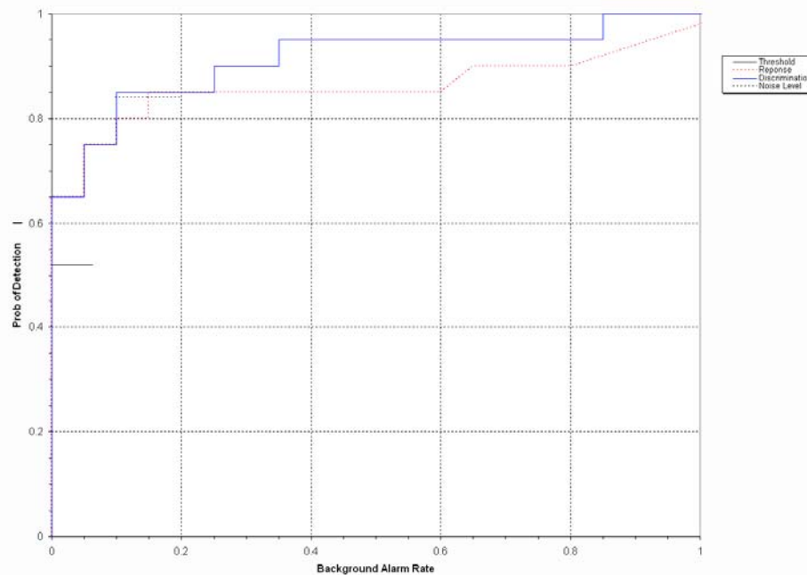
Figure 5. EM61 MKII/towed array blind grid probability of detection for response and discrimination stages versus their respective probabilities of background alarm for all ordnance larger than 20 mm.
