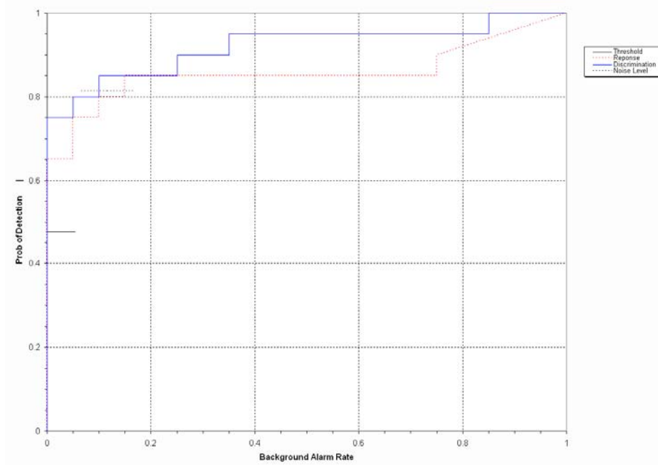
Figure 3. EM61 MKII/towed array blind grid probability of detection for response and discrimination stages versus their respective probability of background alarm over all ordnance categories combined.
