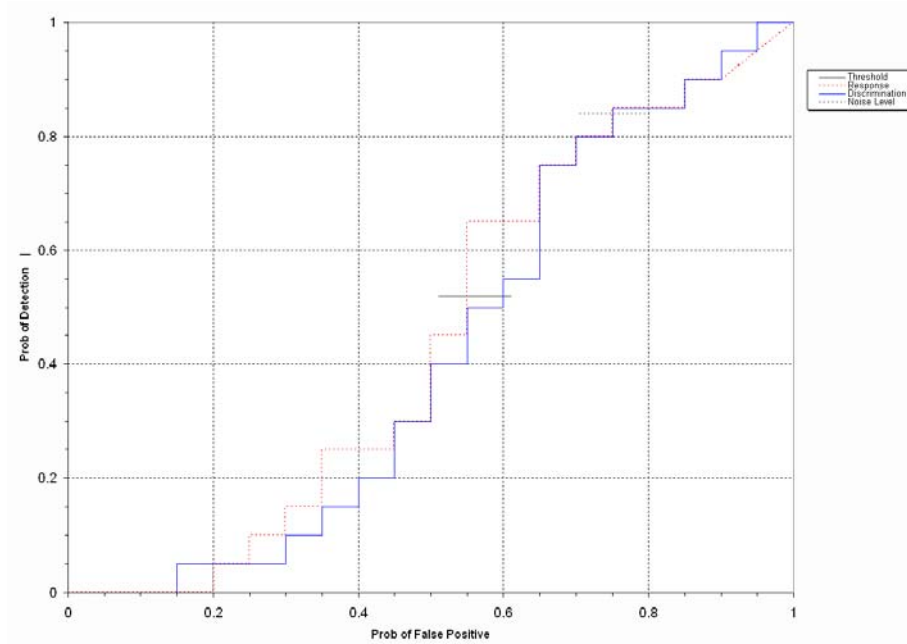
Figure 4. EM61 MKII/towed array blind grid probability of detection for response and discrimination stages versus their respective probability of false positive for all ordnance larger than 20 mm.
