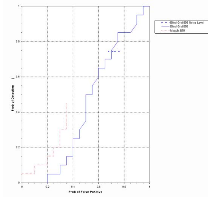
Figure 6. EM61 MKII/pushcart P_d^{\text{res}} stages versus the respective P_{\text{fp}} over all ordnance categories combined.
