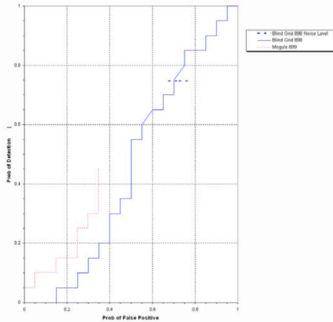
Figure 8. EM61 MKII/pushcart P_d^{\text{res}} versus the respective P_{\text{fp}} for ordnance larger than 20 mm.
