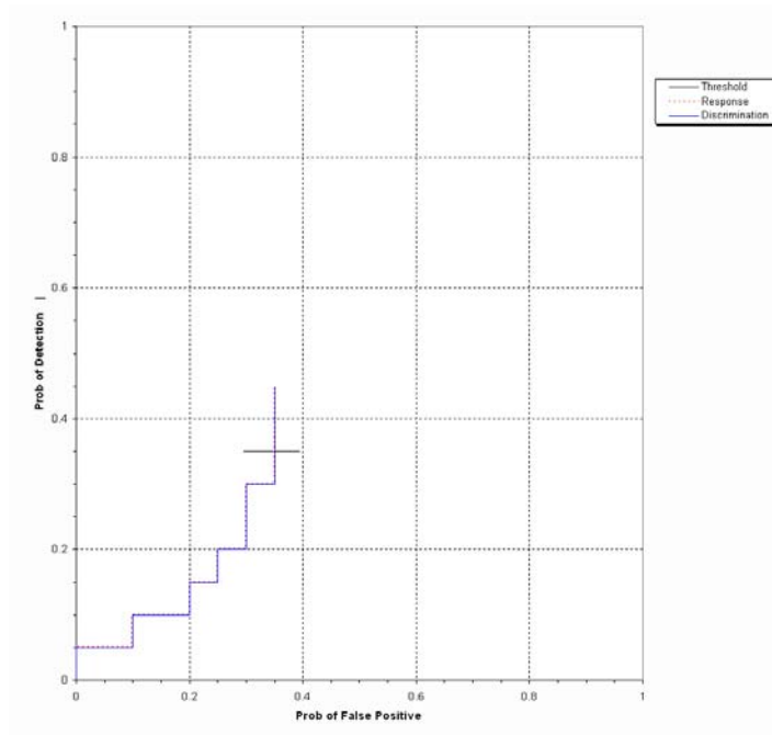
Figure 2. EM61 MKII/pushcart mogul probability of detection for response and discrimination stages versus their respective probability of false positive over all ordnance categories combined.
