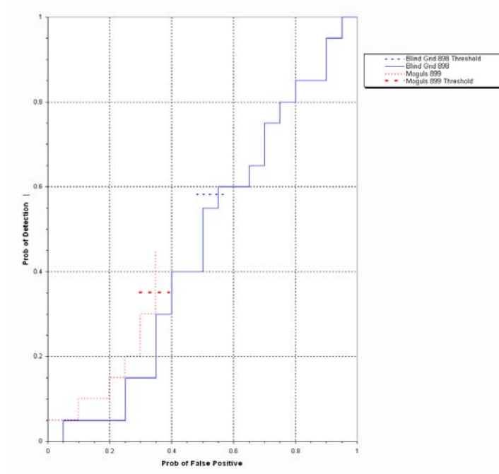
Figure 7. EM61 MKII/pushcart P_d^{\text{disc}} versus the respective P_{\text{fp}} over all ordnance categories combined.
