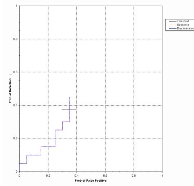
Figure 4. EM61 MKII/pushcart mogul probability of detection for response and discrimination stages versus their respective probability of false positive for all ordnance larger than 20 mm.
