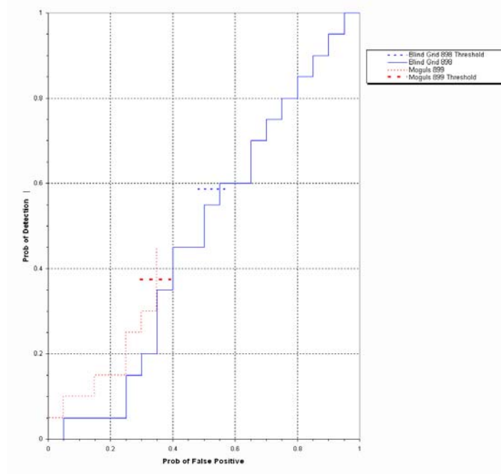
Figure 9. EM61 MKII/pushcart P_d^{\text{disc}} versus the respective P_{\text{fp}} for ordnance larger than 20 mm.
