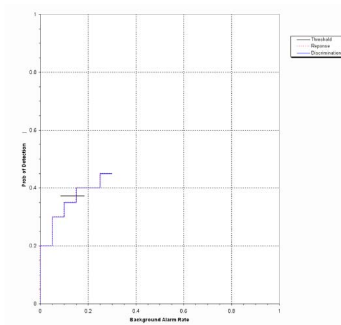
Figure 5. EM61 MKII/pushcart mogul probability of detection for response and discrimination stages versus their respective background alarm rate for all ordnance larger than 20 mm.
