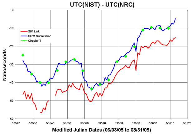
Figure 7. UTC(NIST) – UTC(NRC) comparison.
