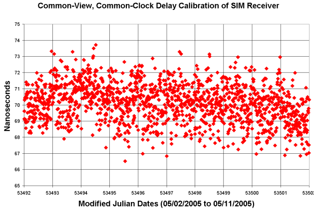
Figure 4. Data from common-clock calibration of the receiver delay.
