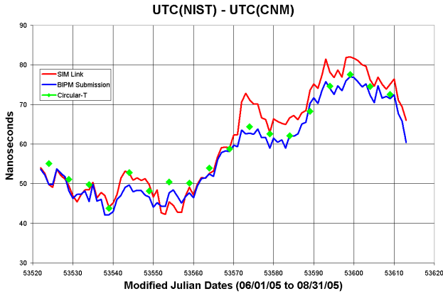
Figure 6. UTC(NIST) – UTC(CNM) comparison.
