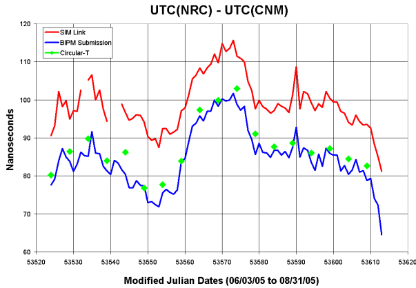
Figure 8. UTC(NRC) – UTC(CNM) comparison.
