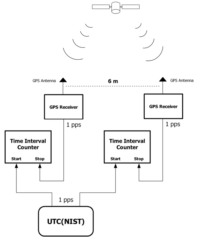
Figure 3. A common-view, common-clock delay calibration.
