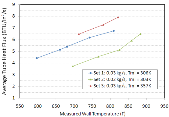
Figure 4. Average tube heat flux as a function of wall temperature for short duration tests in copper tube at varying flow conditions. For similar wall temperature and bulk inlet temperature, Set 2 heat flux is less than Set 1 heat flux due to a lower mass flow rate. Heat transfer for Set 3 is greater than that for Set 1 due to higher inlet bulk fuel temperature, with similar mass flow rate and wall temperature.
