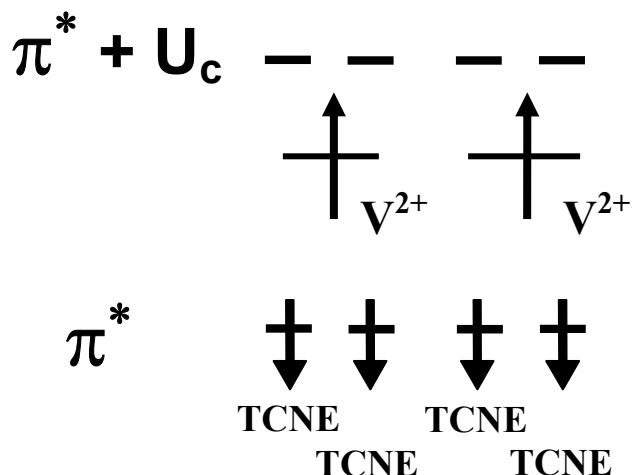
Figure 2.9. 1-D spatial distribution and relative energy alignment of the V^{2+} 3d and [TCNE]^{-} \pi^* levels in V[TCNE]_{-2} . Each [TCNE]^{-} \pi^* orbital can accommodate two electrons with antiparallel spins, but the addition of an electron to the singly occupied molecular orbital carries with it an additional Coulomb repulsion energy, U_c . The \pi^* + U_c , a separate sub-band as viewed in this model, level is involved in hopping charge transport along with the V 3d level.
