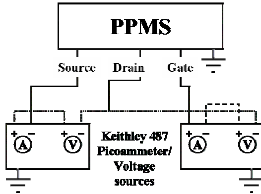
Figure 3.7. Wiring schematic for testing the V[TCNE]_{-2} field-effect transistors. The Keithley picoammeter triaxial cable shields are grounded through the PPMS cable shield ground. The difference in the line types is not to indicate differences in the wire types used but only to indicate the connectivity of the setup.
