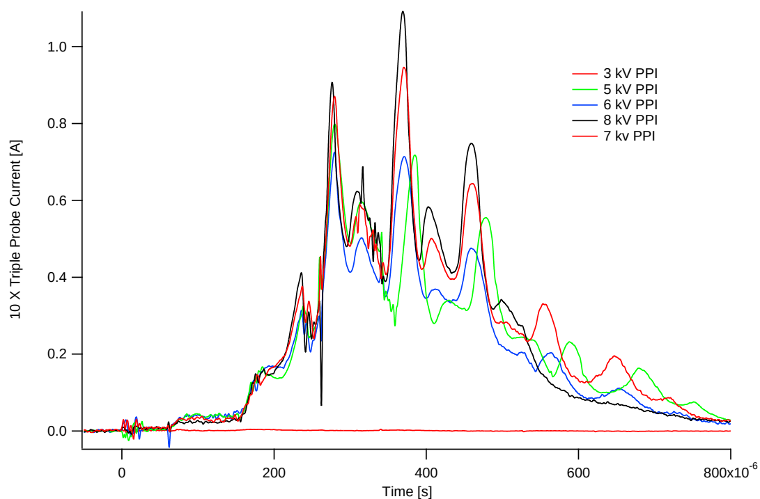
Figure 4.19: Downstream current collection data for a 14-mTorr, 750-V, main bank discharge for various PPI glow discharge voltages
