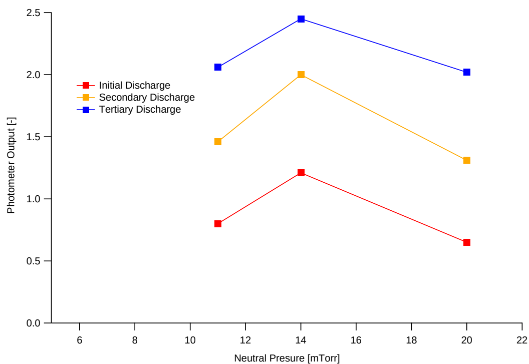
Figure 7.26: Peak photometer results as a function of background pressure for multiple discharges at 14 mTorr and 950 V
