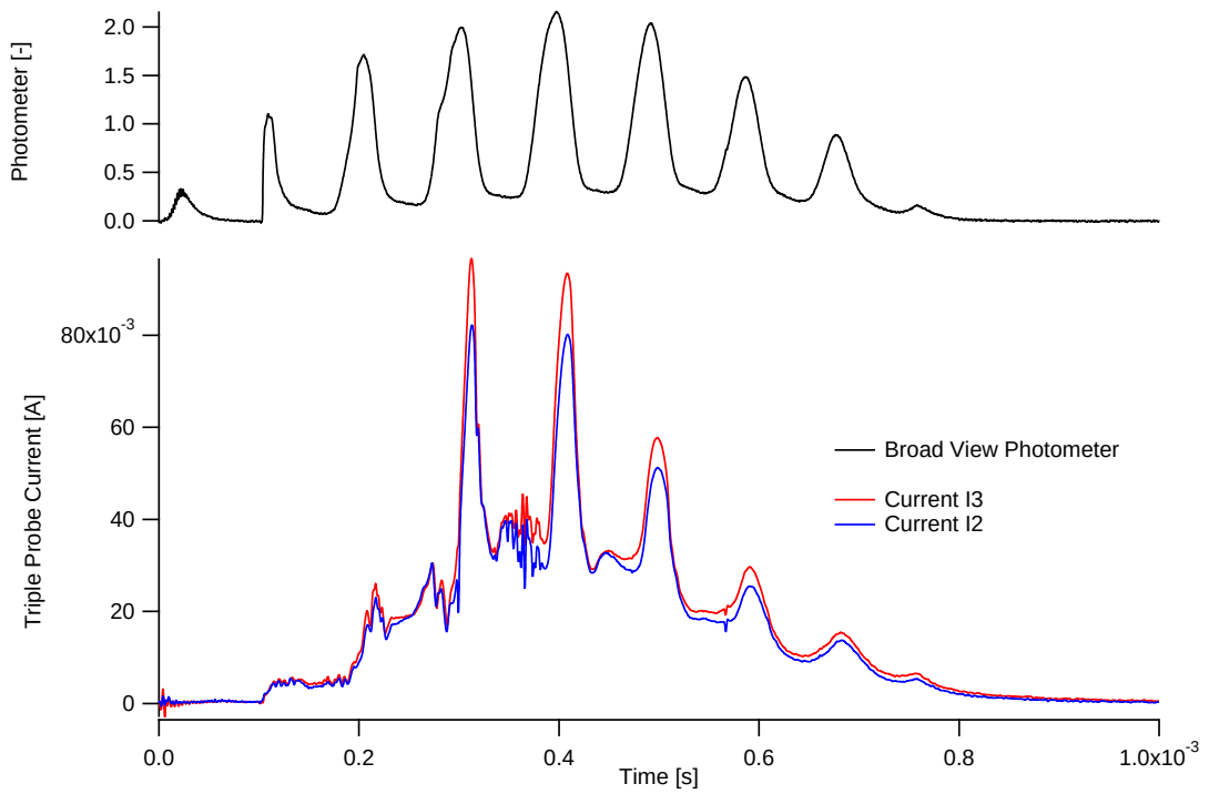
Figure 7.5: Collected triple probe current (both I_2 and I_3 , see Figure 2.42) for a typical 850-V, 185- \mu s, 14-mTorr argon discharge
