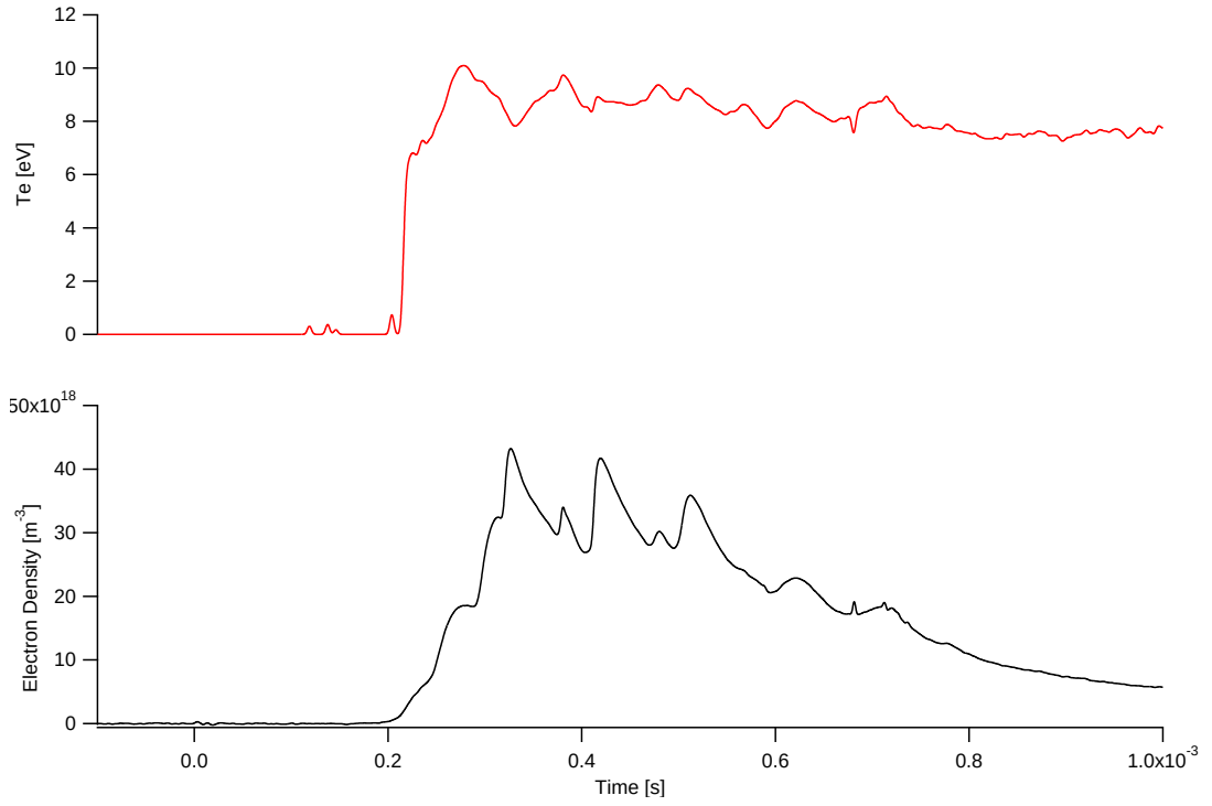
Figure 7.63: Detailed time evolution of electron density and temperature at Position 2 for an 850-V, 185- \mu s, 10-mTorr xenon discharge
