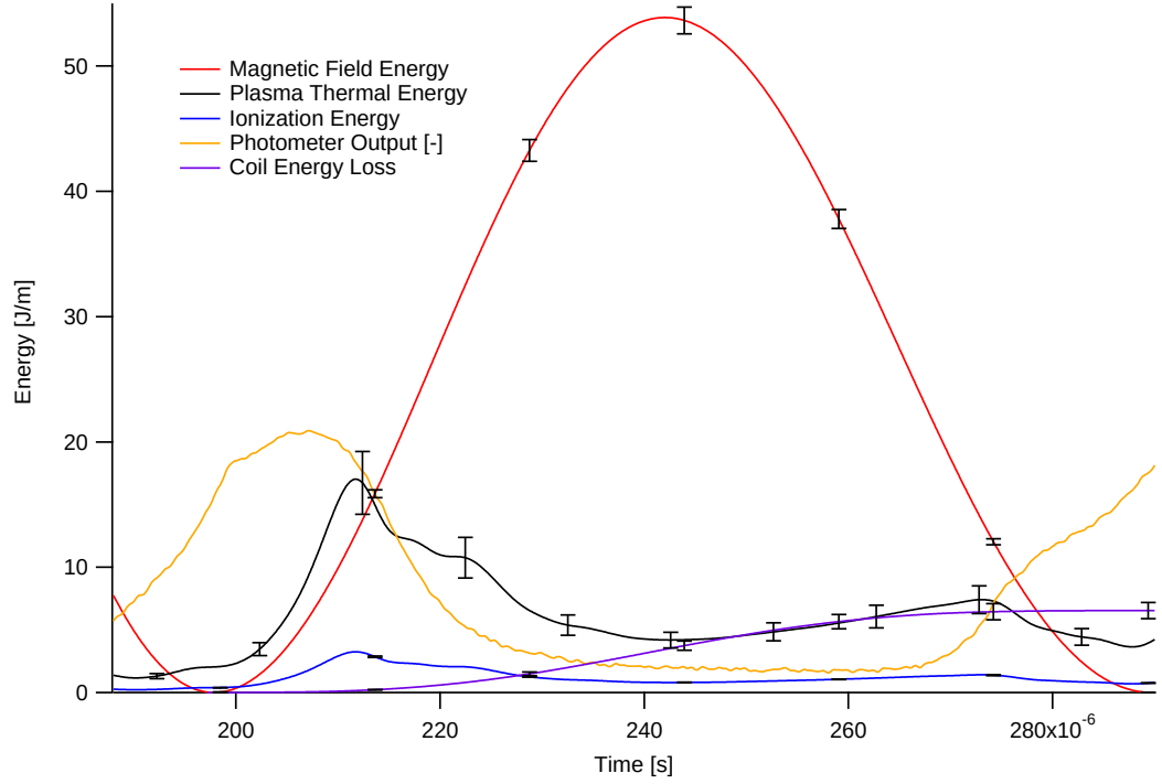
Figure 8.14: Instantaneous energy contained in the annular discharge region (per unit length) for a 185\text{-}\mu\text{s} , 14\text{-mTorr} , 950\text{-V} argon discharge showing plasma, ionization, magnetic, and coil dissipation energies as well as wide-angle photometer output
