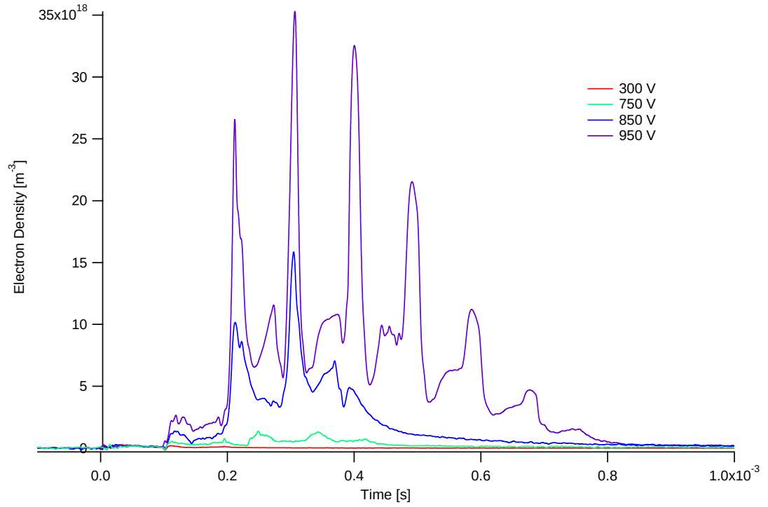
Figure 7.38: Summary of plasma density results at Position 3 for 185- \mu\text{s} , 14-mTorr argon discharges for various energies
