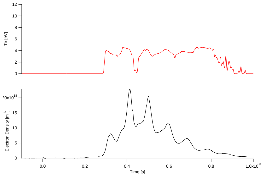
Figure 7.19: Detailed time evolution of electron density and temperature at Position 1 for a 950-V, 185- \mu\text{s} , 20-mTorr argon discharge
