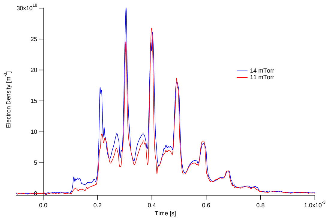
Figure 7.40: Summary of plasma density results at Position 3 for 185- \mu\text{s} , 950-V argon discharges for various neutral fill pressures
