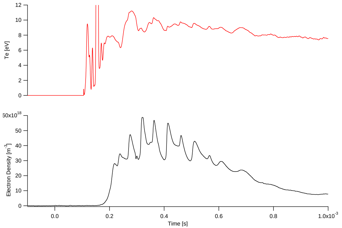
Figure 7.64: Detailed time evolution of electron density and temperature at Position 2 for a 950-V, 185- \mu s, 10-mTorr xenon discharge
