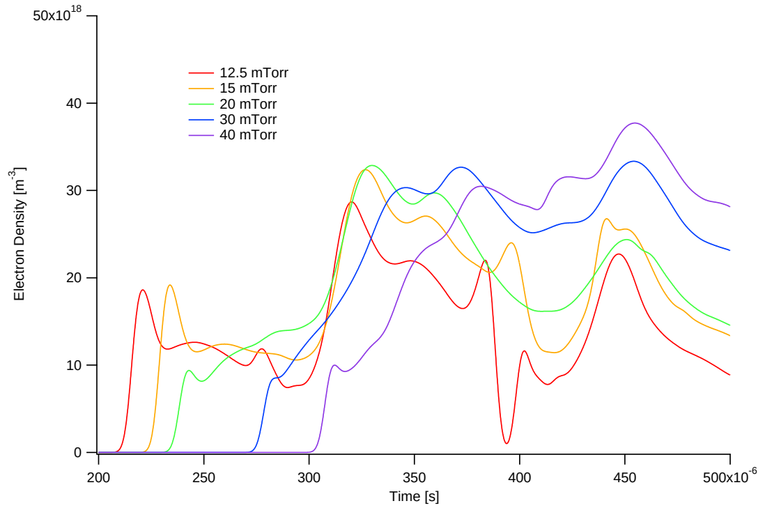
Figure 6.17: Close up of a 900-V, 250- \mu\text{s} discharge showing electron density for various discharge pressures at Position 0
