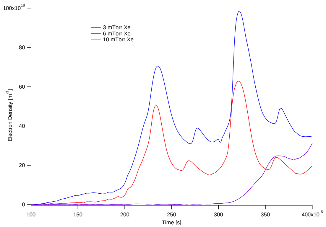
Figure 7.59: Close view of plasma density results at Position 1 for 185- \mu s, 950-V xenon discharges for various neutral fill pressures showing the primary and secondary discharges
