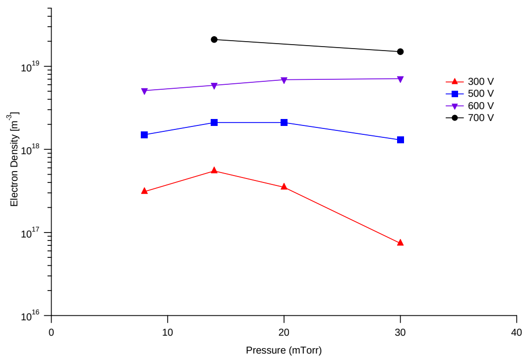
Figure 5.12: Peak Electron densities measured as a function of background pressure for multiple discharge voltages. From 200–400 \mu s
