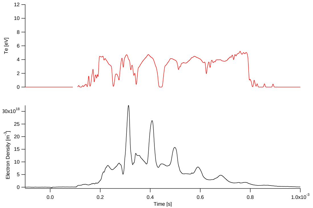
Figure 7.13: Detailed time evolution of electron density and temperature at Position 1 for a 950-V, 185- \mu s, 14-mTorr argon discharge
