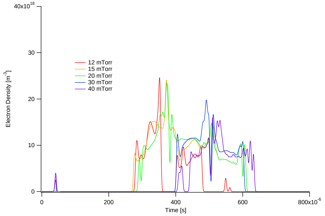
Figure 6.15: A 500-V, 250- \mu s, 15-mTorr discharge showing electron density for various discharge pressures at Position 0
