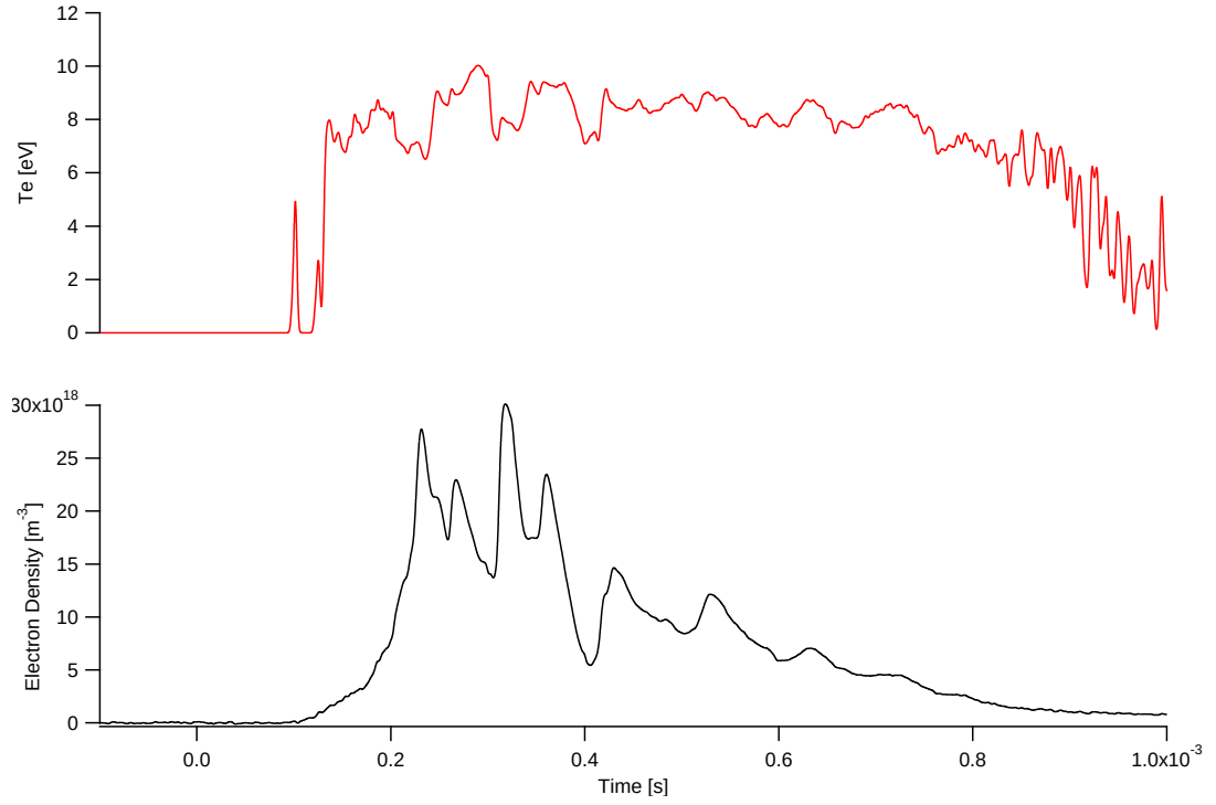
Figure 7.60: Detailed time evolution of electron density and temperature at Position 2 for an 850-V, 185- \mu s, 3-mTorr xenon discharge
