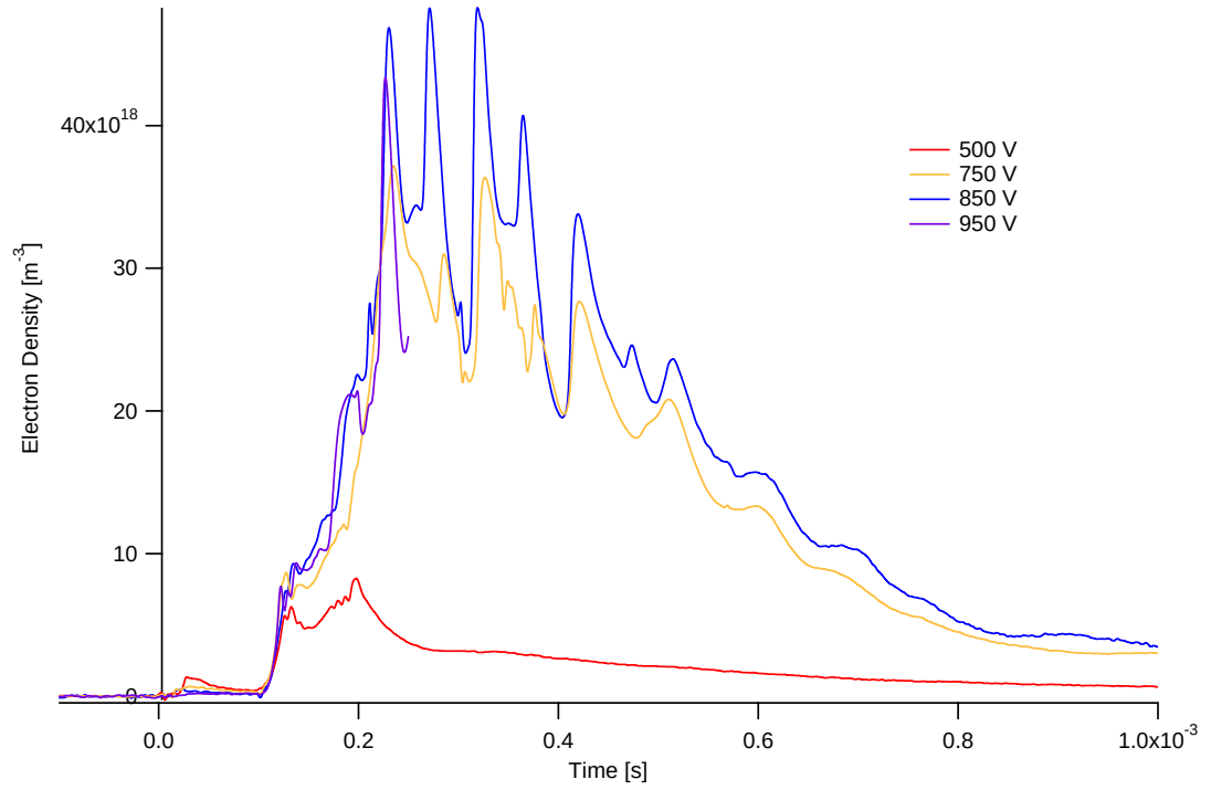
Figure 7.66: Summary of plasma density results at Position 2 for 185- \mu s, 6-mTorr xenon discharges for various energies. Note that the 950-V, 6-mTorr case is not complete due to a data collection error
