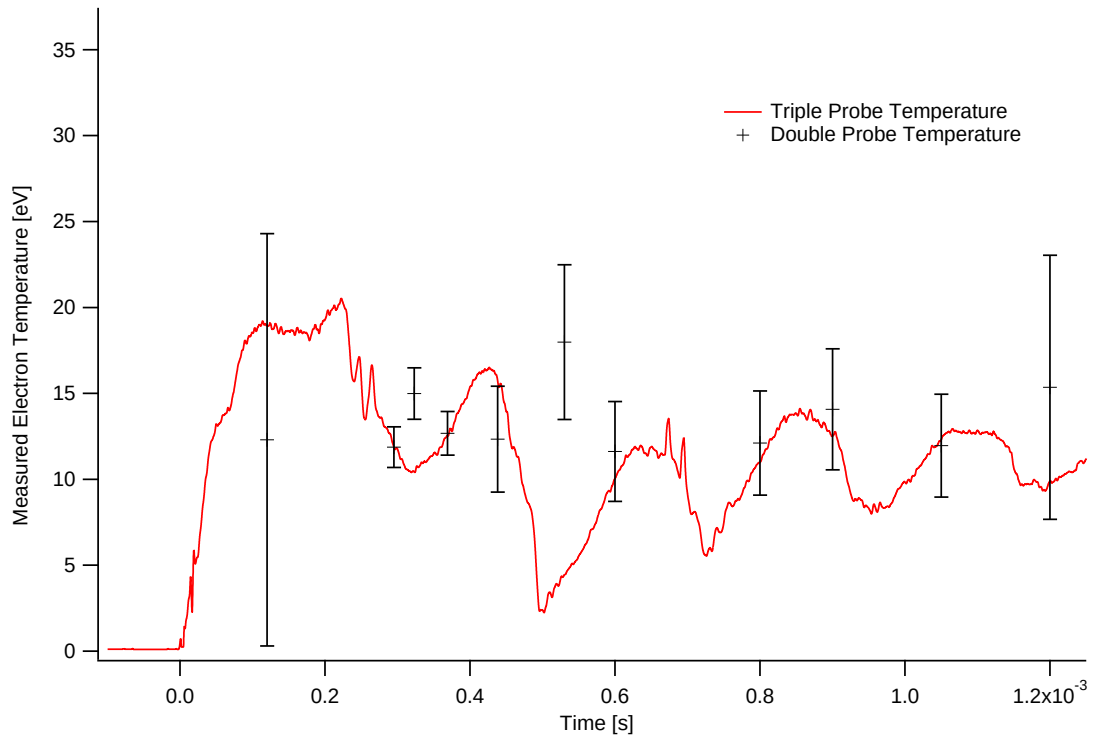
Figure 5.9: Comparison of triple probe T_e to a congrate double probe temperature measurement at the highest confidence points
