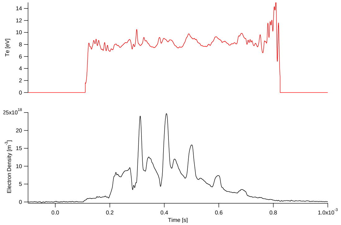
Figure 7.28: Detailed time evolution of electron density and temperature at Position 2 for a 950-V, 185- \mu\text{s} , 14-mTorr argon discharge
