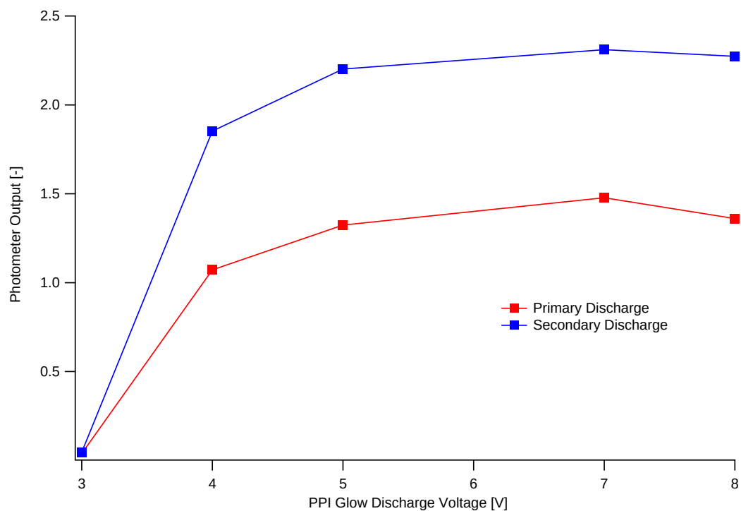
Figure 4.18: Summary of peak photometer data for various PPI glow discharge and 750-V main bank discharges
