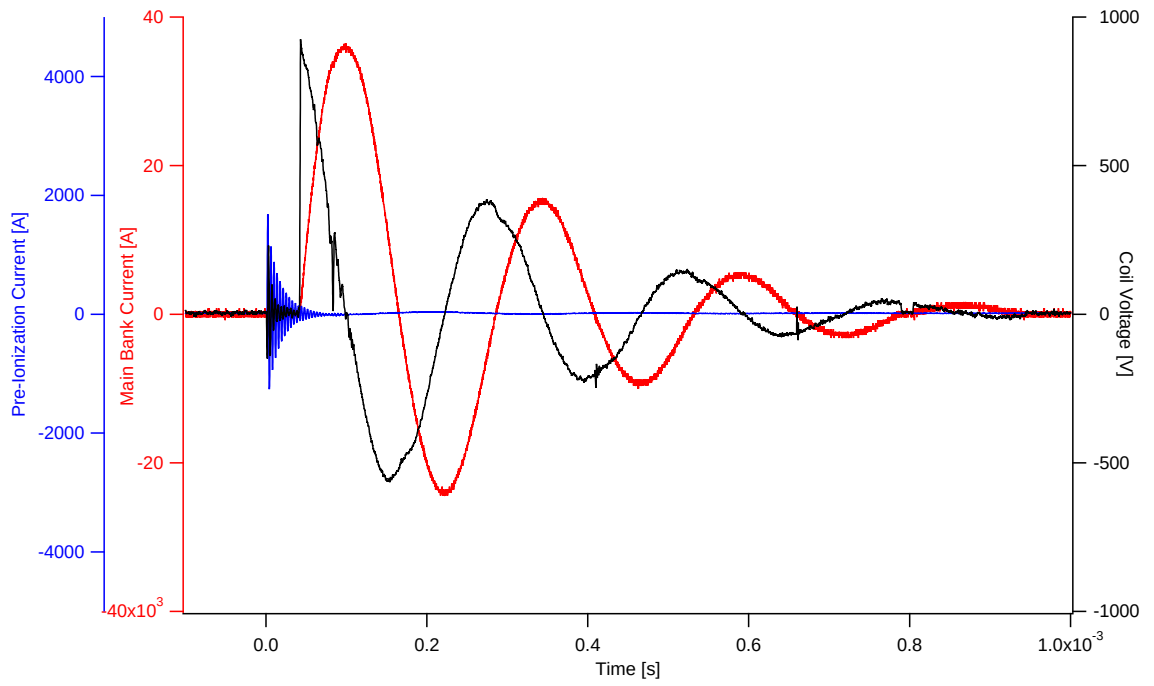
Figure 6.1: A 900-V discharge showing total discharge current (both coils), pre-ionization current, and instantaneous coil voltage for a 250\text{-}\mu\text{s} discharge
