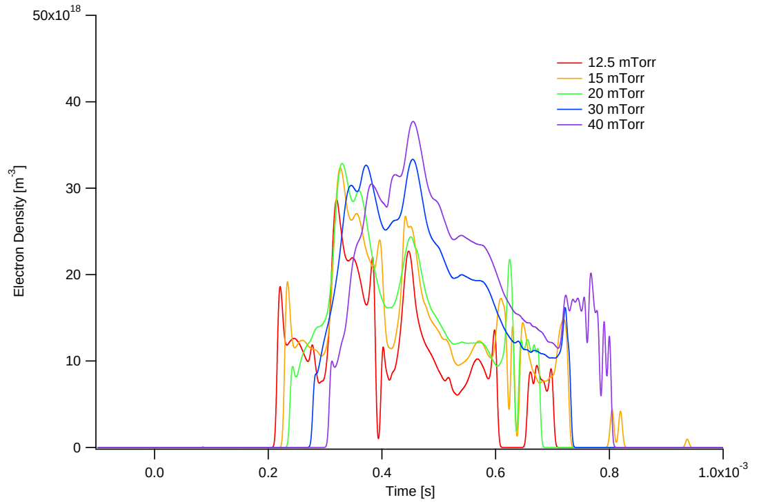
Figure 6.16: A 900-V, 250- \mu s, 15-mTorr discharge showing electron density at Position 0
