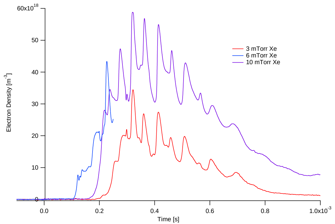
Figure 7.68: Summary of plasma density results at Position 2 for 185\text{-}\mu\text{s} , 950-V xenon discharges for various neutral fill pressures
