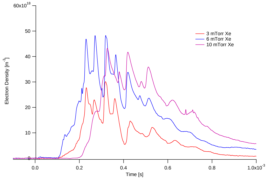
Figure 7.67: Summary of plasma density results at Position 2 for 185- \mu s, 850-V xenon discharges for various neutral fill pressures
