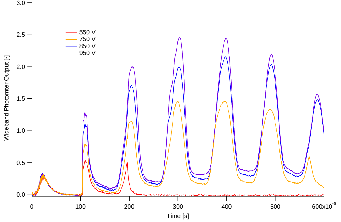
Figure 7.24: Detailed time evolution of wide-angle photometer output at Position 1 for a 950-V, 185- \mu s, 14-mTorr argon discharge
