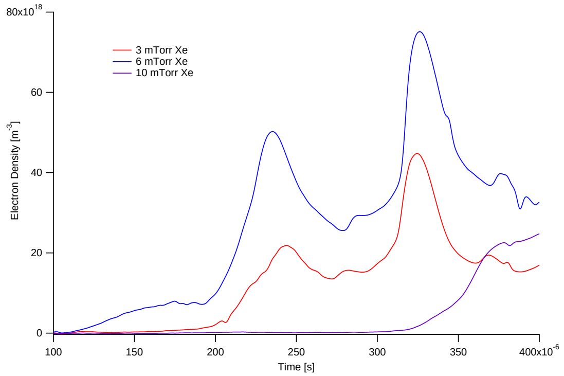
Figure 7.57: Close view of plasma density results at Position 1 for 185- \mu\text{s} , 850-V xenon discharges for various neutral fill pressures showing the primary and secondary discharges
