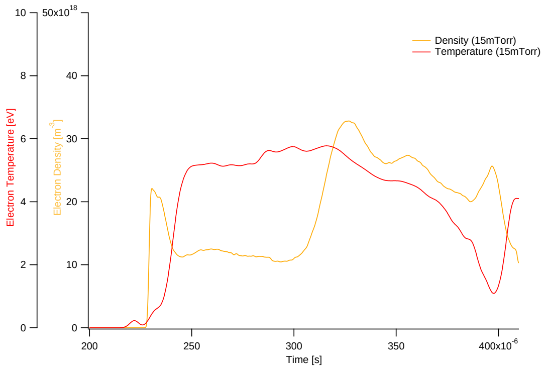
Figure 6.18: A 900-V, 250- \mu\text{s} , 15-mTorr discharge showing simultaneous electron density and temperature for various discharge pressures at Position 0
