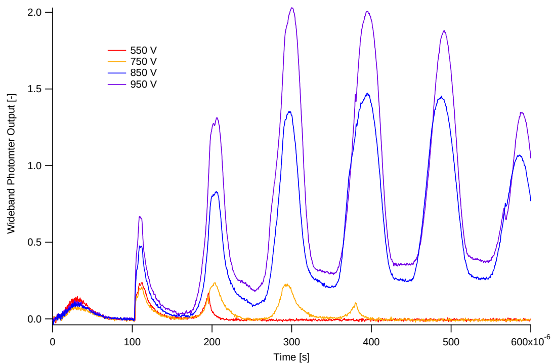
Figure 7.25: Detailed time evolution of wide-angle photometer output at Position 1 for a 950-V, 185- \mu s, 20-mTorr argon discharge
