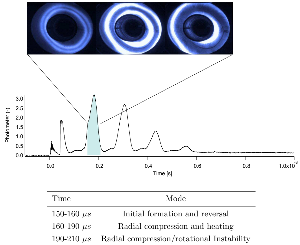
Figure 6.3: DICAM photos and descriptions of typical formation and compression regimes during a 250- \mu s discharge
