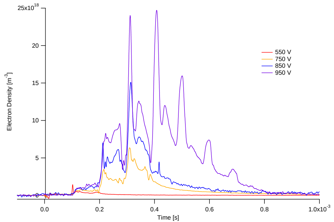
Figure 7.29: Summary of plasma density results at Position 2 for 185- \mu\text{s} , 14-mTorr argon discharges for various energies
