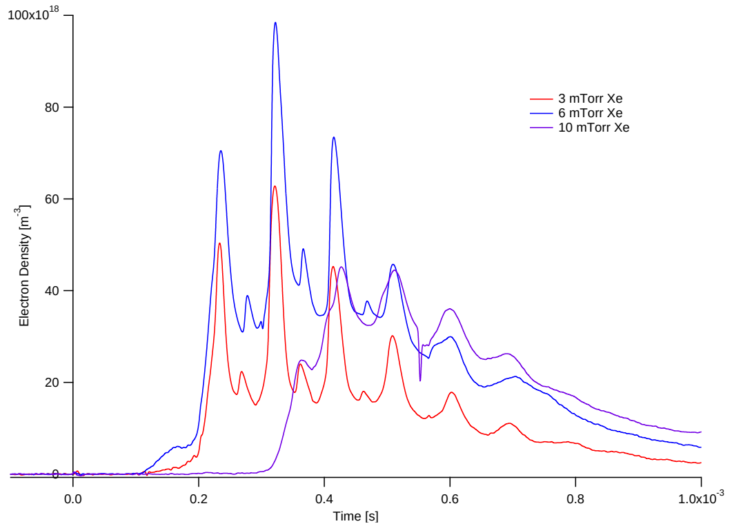
Figure 7.58: Summary of plasma density results at Position 1 for 185- \mu\text{s} , 950-V xenon discharges for various neutral fill pressures
