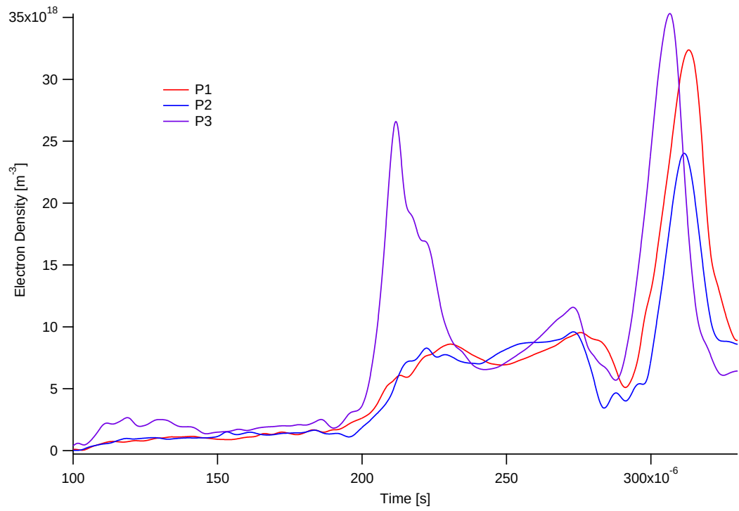
Figure 7.42: Detailed axial density scans for 185- \mu\text{s} , 14-mTorr, 950-V argon discharges showing initial ionization, primary, and secondary discharges
