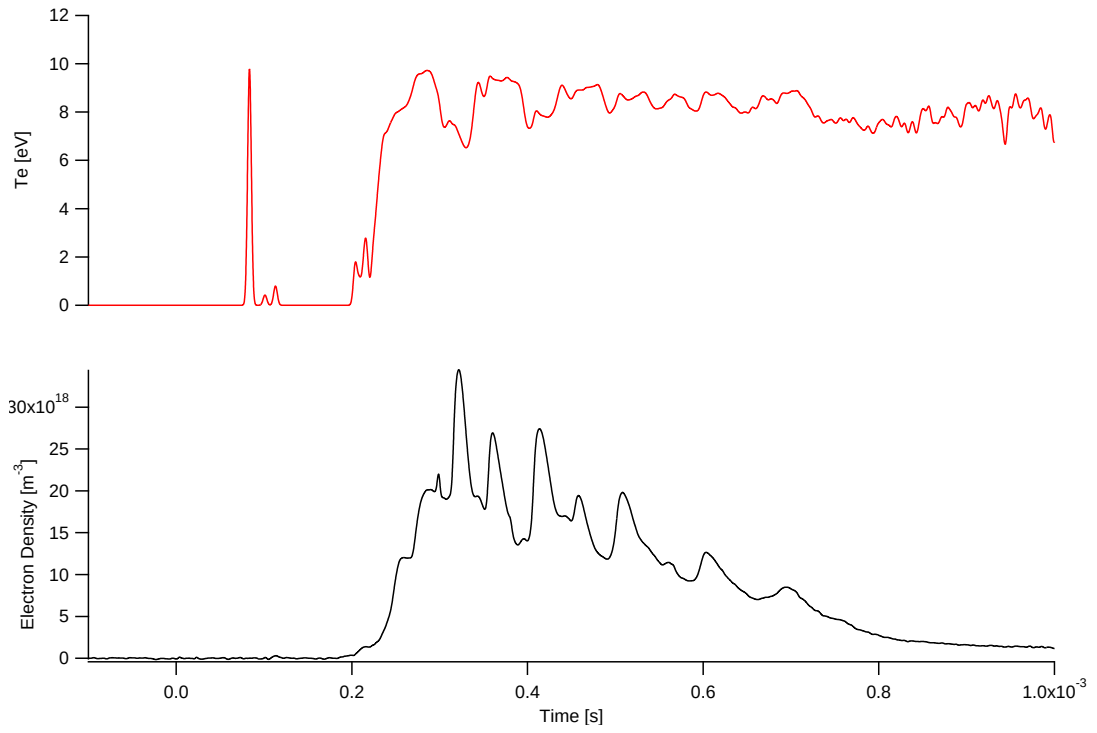
Figure 7.61: Detailed time evolution of electron density and temperature at Position 2 for a 950-V, 185- \mu s, 3-mTorr xenon discharge
