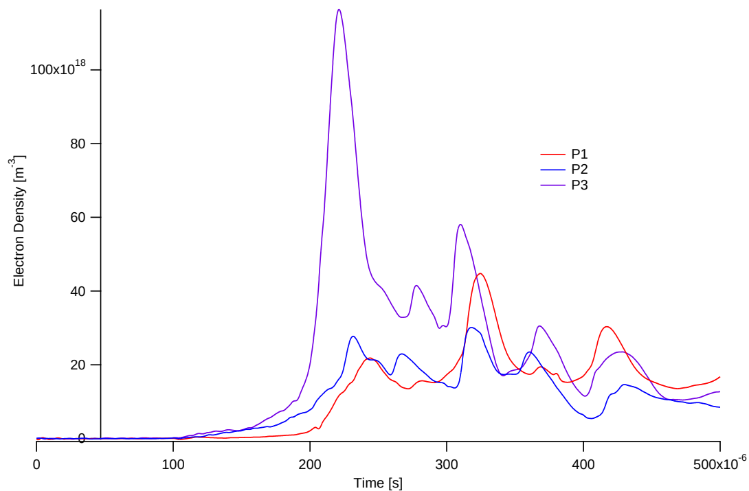
Figure 7.75: Detailed axial density scans for 185- \mu\text{s} , 3-mTorr, 850-V xenon discharges showing initial ionization, primary, and secondary discharges
