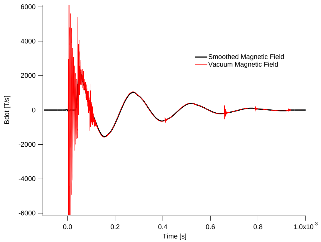
Figure 2.27: Raw B-dot probe data and filtered data for a 900-V, 250\text{-}\mu\text{s} discharge
