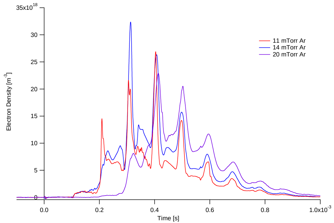
Figure 8.11: Summary of plasma density results at Position 1 for 185\text{-}\mu\text{s} , 950-V argon discharges for various neutral fill pressures
