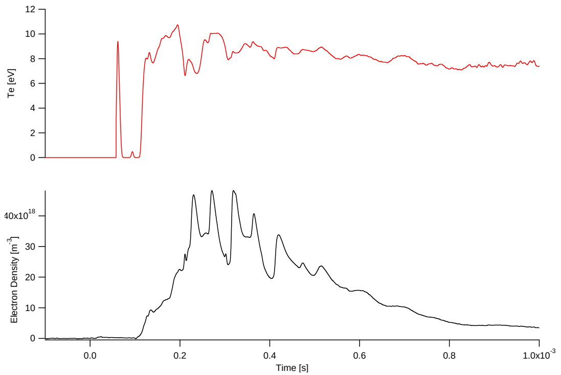
Figure 7.62: Detailed time evolution of electron density and temperature at Position 2 for an 850-V, 185- \mu s, 6-mTorr xenon discharge
