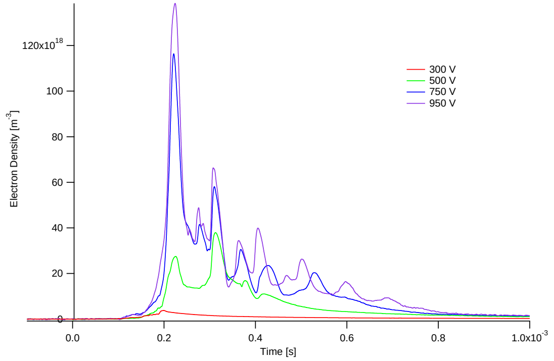
Figure 7.70: Summary of plasma density results at Position 3 for 185- \mu s, 3-mTorr xenon discharges for various energies
