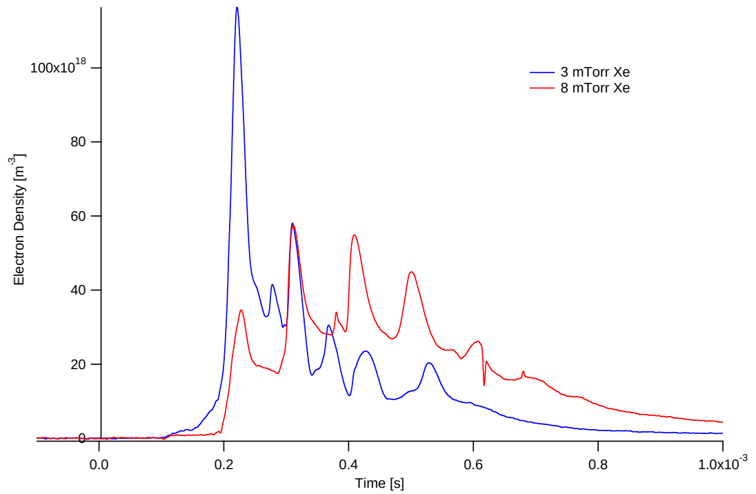
Figure 7.71: Summary of plasma density results at Position 3 for 185- \mu s, 850-V xenon discharges for various neutral fill pressures
