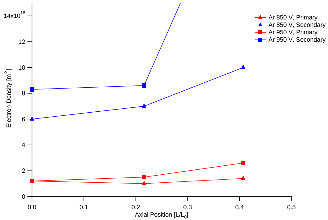
Figure 8.10: Close view of the peak densities within the first 350 \mu\text{s} at Positions 1, 2, and 3 for 14-mTorr discharges at 850 V and 950 V as a function of axial position
