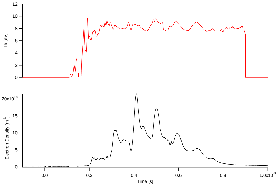
Figure 7.31: Detailed time evolution of electron density and temperature at Position 2 for a 950-V, 185 \mu s, 20-mTorr argon discharge
