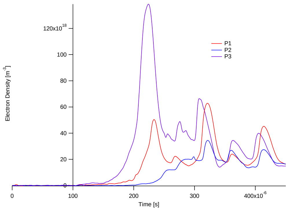
Figure 7.76: Detailed axial density scans for 185- \mu\text{s} , 3-mTorr, 950-V xenon discharges showing initial ionization, primary, and secondary discharges
