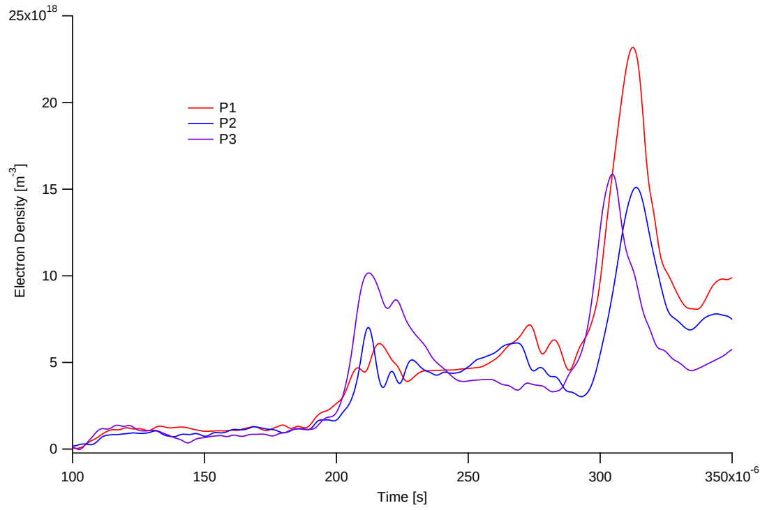
Figure 7.41: Detailed axial density scans for 185- \mu\text{s} , 14-mTorr, 850-V argon discharges showing initial ionization, primary, and secondary discharges
