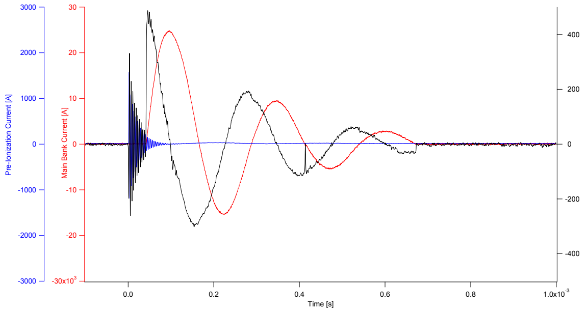
Figure 6.2: A 500-V discharge showing total discharge current (both coils), pre-ionization current, and instantaneous coil voltage for a 250\text{-}\mu\text{s} discharge
