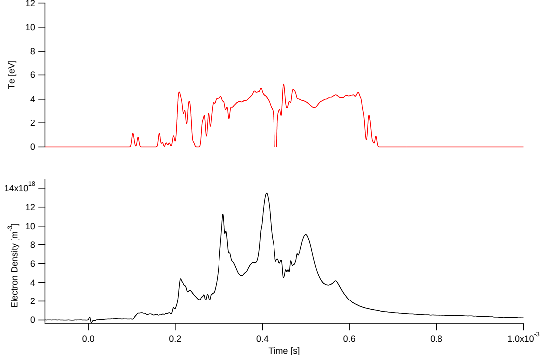
Figure 7.11: Detailed time evolution of electron density and temperature at Position 1 for an 750-V, 185- \mu s, 14-mTorr argon discharge
