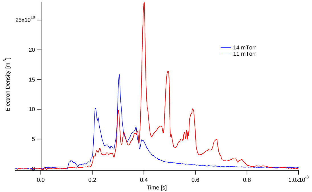
Figure 7.39: Summary of plasma density results at Position 3 for 185- \mu\text{s} , 850-V argon discharges for various neutral fill pressures
