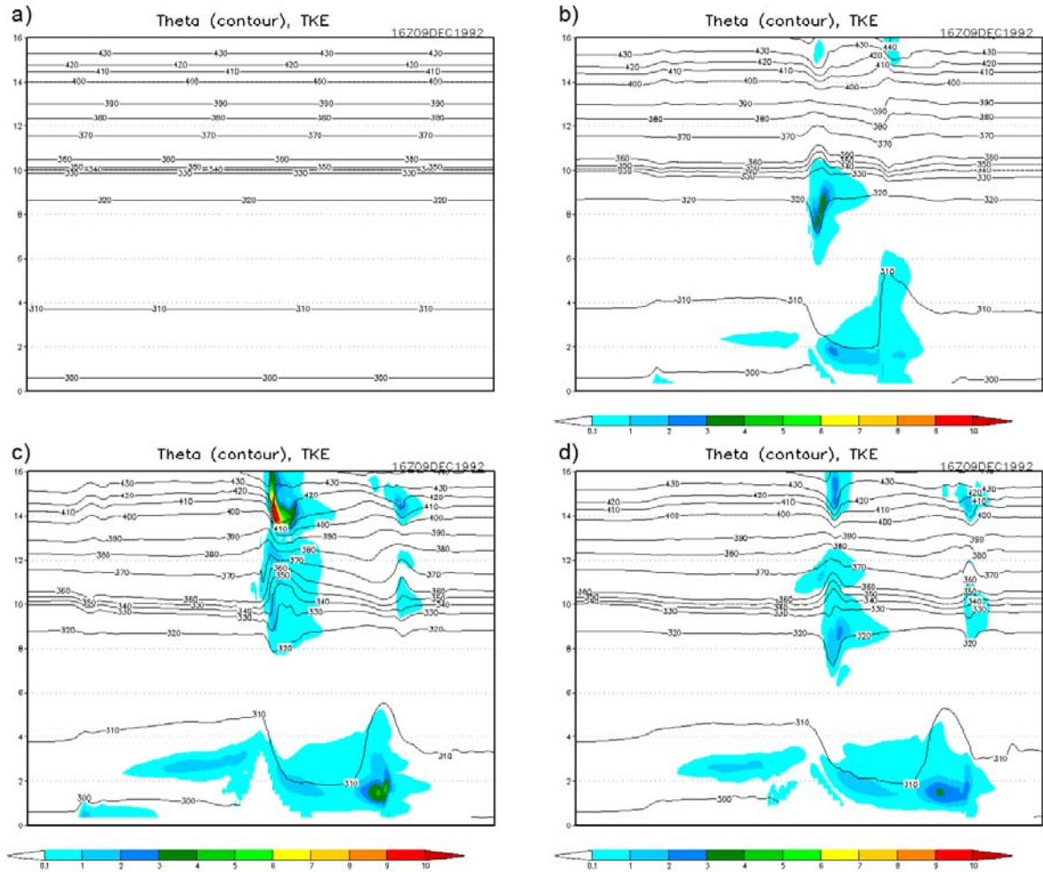
Figure 4.10: Same as Fig. 4.7, except for (a) TCF, (b) TCS, (c) TCH, and (d) TCW simulations.
