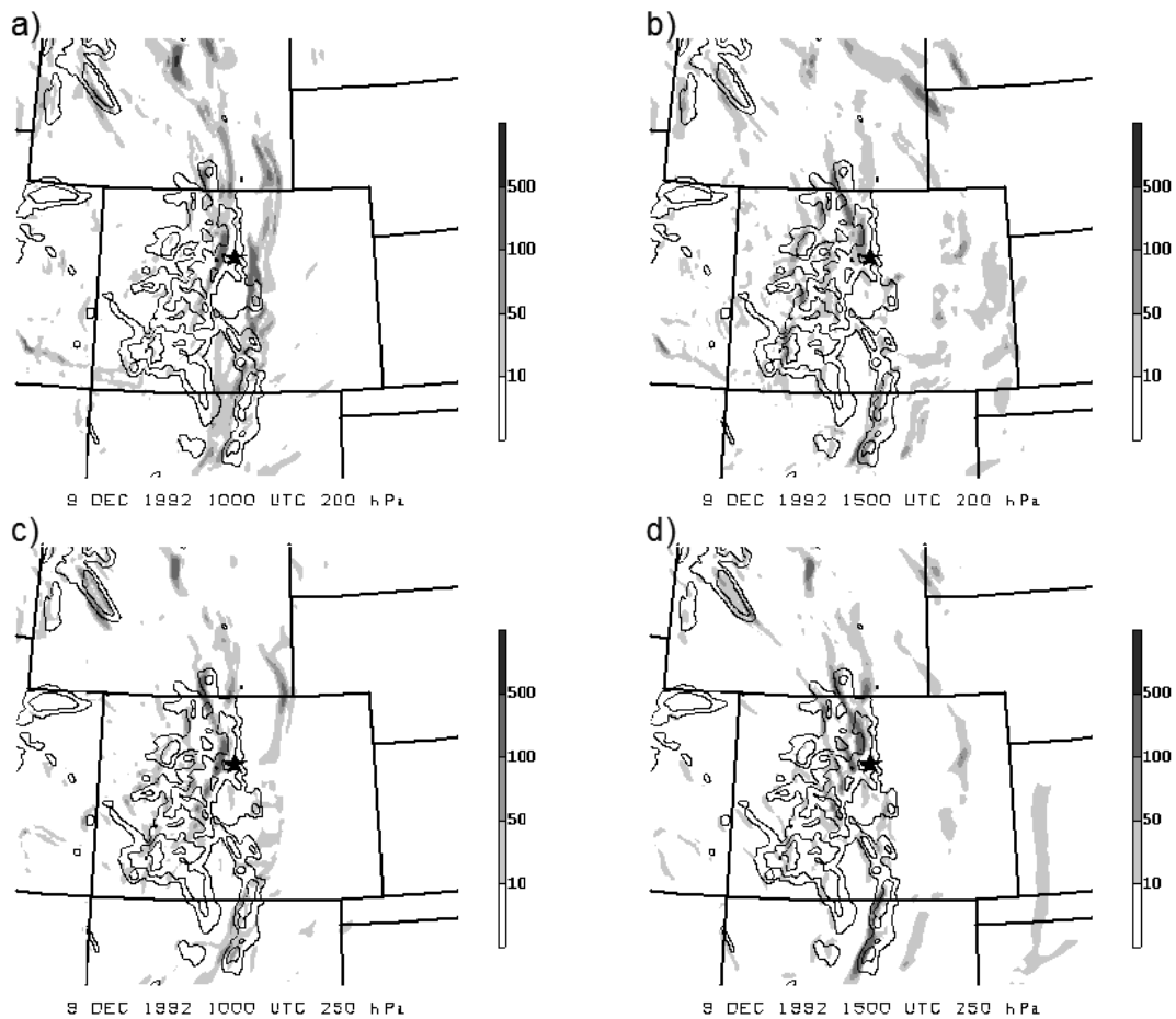
Figure A.7: Simulated 200 hPa GEMPAK-derived horizontal frontogenesis function ( \text{K } 100 \text{ km}^{-1} \text{ 3hr}^{-1} , shaded) at (a) 1000 UTC and (b) 1500 UTC and at 250 hPa at (c) 1000 UTC and (d) 1500 UTC 9 December 1992. Terrain contours at 2.5, 3, and 3.5 km. From 6 km NHMASS full-terrain simulation. Aircraft accident location denoted by star.
