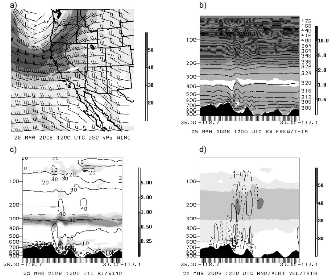
Figure 3.11: (a) Winds ( \text{ms}^{-1} ) at 250 hPa from 18 km WRF simulation. Vertical west-east cross-section of (b) potential temperature (contoured) and N^2 (shaded, \text{s}^{-1} \times 10^{-4} ), (c) Ri (shaded) and wind speed ( \text{ms}^{-1} , contoured), and (d) wind speed ( \text{ms}^{-1} , shaded) and vertical velocity ( \text{ms}^{-1} , contoured, dashed for downward vertical motion), from 2 km WRF simulation valid 1200 UTC 25 March 2006. Cross-sections along the heavy white line in (a). Vertical scale is hPa and horizontal scale is grid spacing (2 km per tick).
