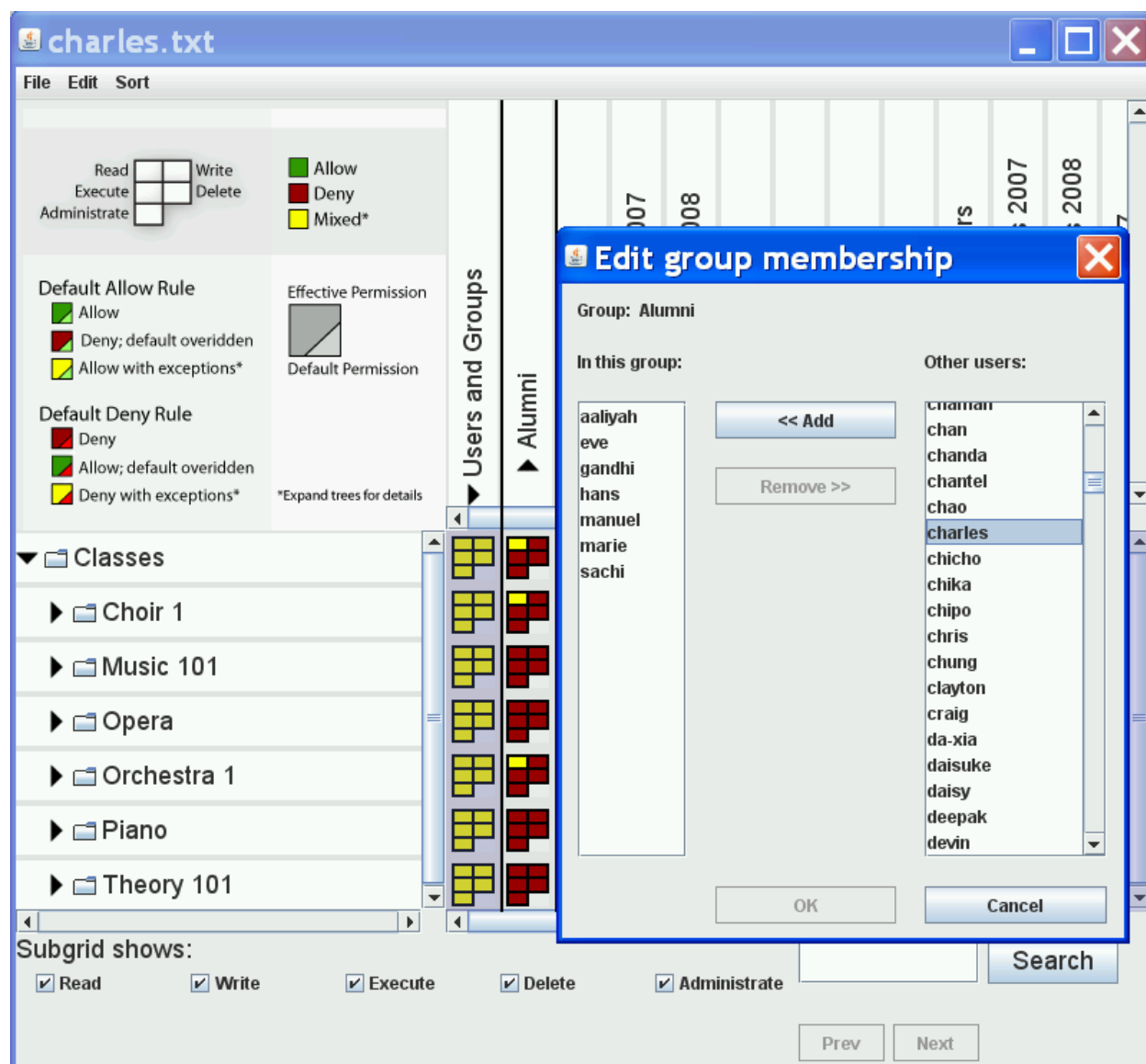
Figure 7.1: A screenshot of the Grid interface with the edit group membership dialog showing. The dialog allows the policy author to add users to a group or remove them from the group.
