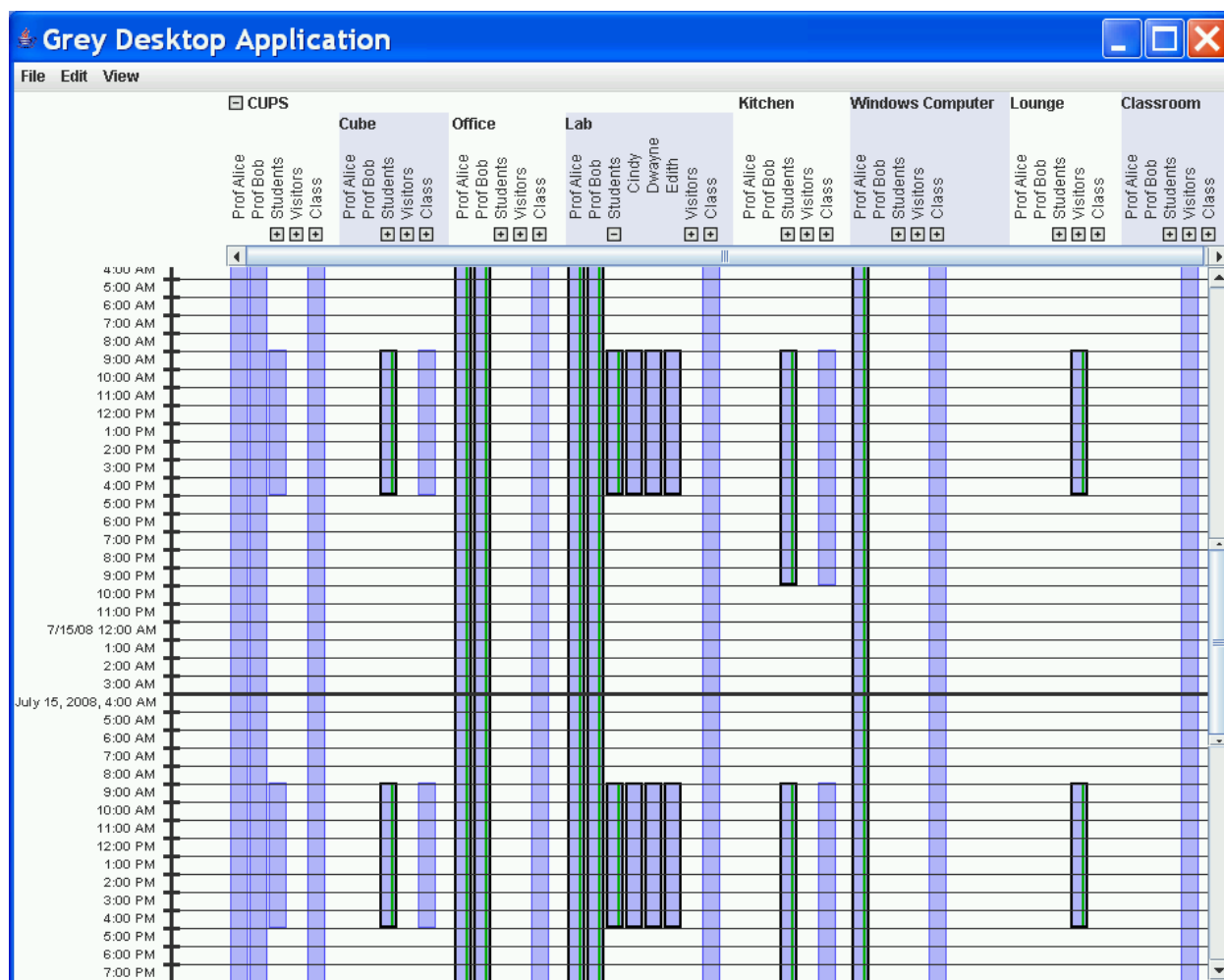
Figure 9.1: A screenshot of our Grey Expandable Grid interface. The Grey Expandable Grid shows how policies with a time attribute can be shown in an Expandable Grid.
