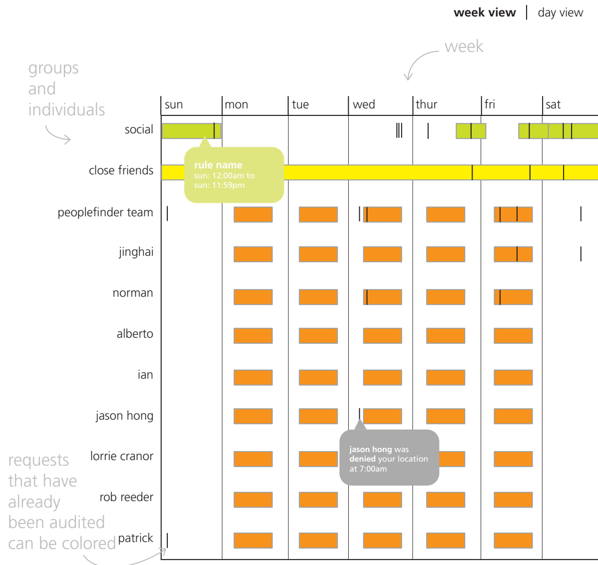
Figure 9.4: A mockup (by Madhu Prabaker) of an Expandable-Grid-based user interface for viewing and editing PeopleFinder location-disclosure policies.
