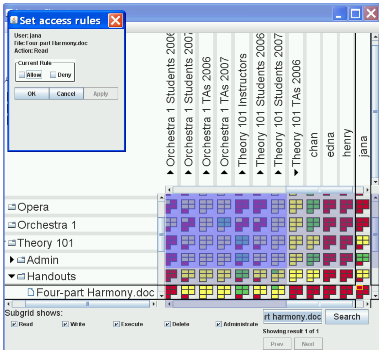
Figure 7.3: Screenshot of the Grid-with-Windows-semantics interface used in Policy Semantics Study #1. Since direct manipulation is not possible with the Windows semantics, the interface shows a dialog box to allow a policy author to set an access rule.
