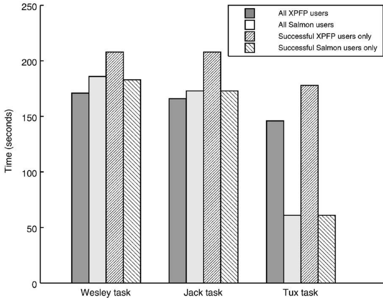
Figure 3.4: Average time to complete Wesley, Jack, and Tux tasks. Successful Salmon users took less time on average than successful XPFP users did, suggesting that Salmon’s accuracy gains were not due simply to a speed-accuracy tradeoff.
