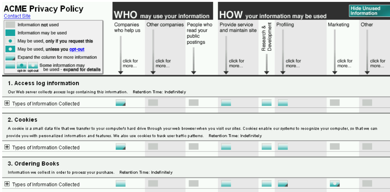
Figure 8.1: Screenshot of the P3P Expandable Grid in unexpanded form. The column groups labeled “WHO” and “HOW” show P3P recipients and purposes, respectively. The rows show three P3P statements with their header boxes and the roots of their data hierarchies (the roots are labeled “Types of information collected”). The column headers and data hierarchies can be expanded and contracted to show more or fewer P3P elements.
