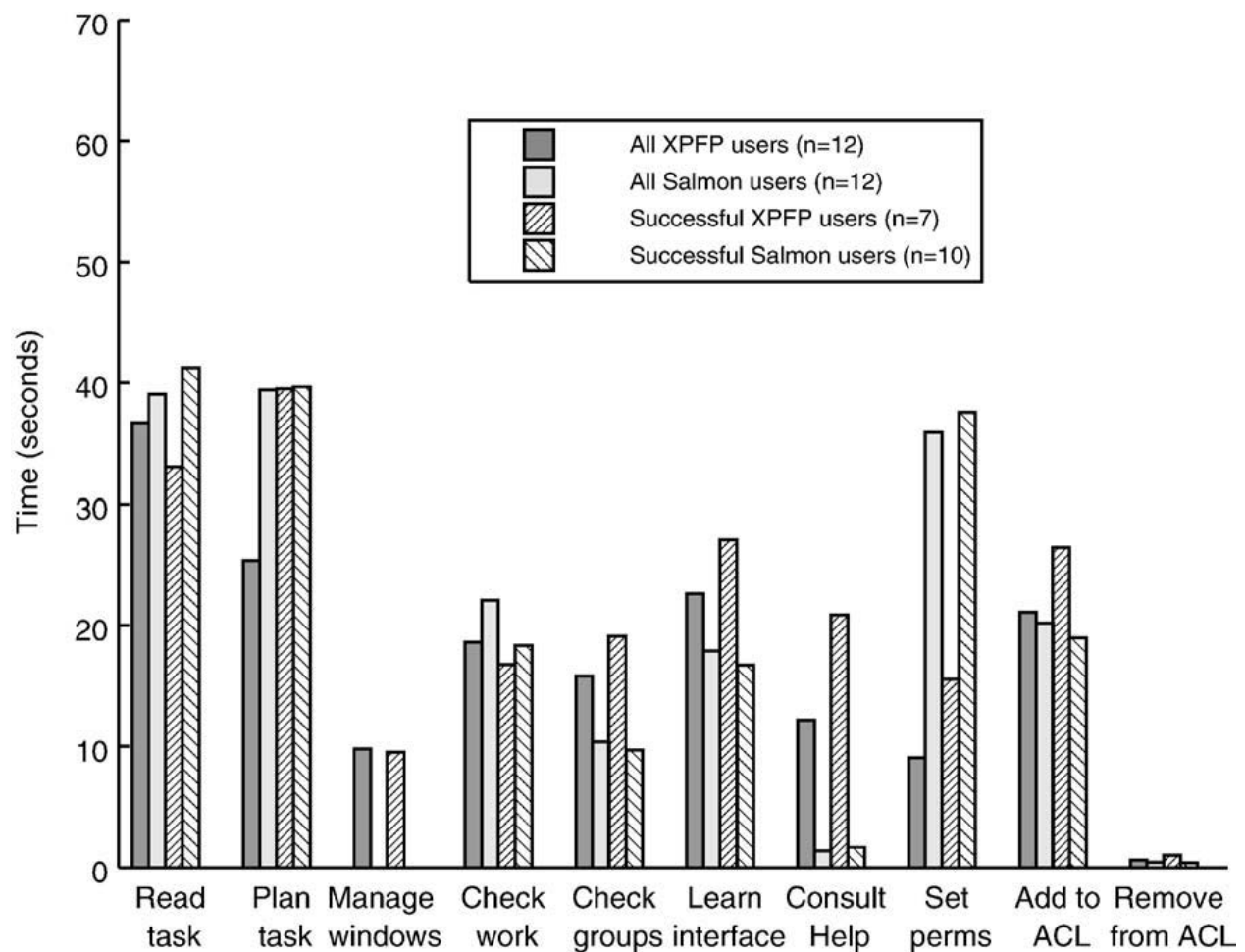
Figure 3.5: Average time spent on each of 10 behaviors identified in the Wesley task by all XPFP and Salmon users combined, whether successful or not, and only successful XPFP and Salmon users. Salmon users spent less time on information-gathering behaviors like check-groups, learn-interface, and consult-help.
