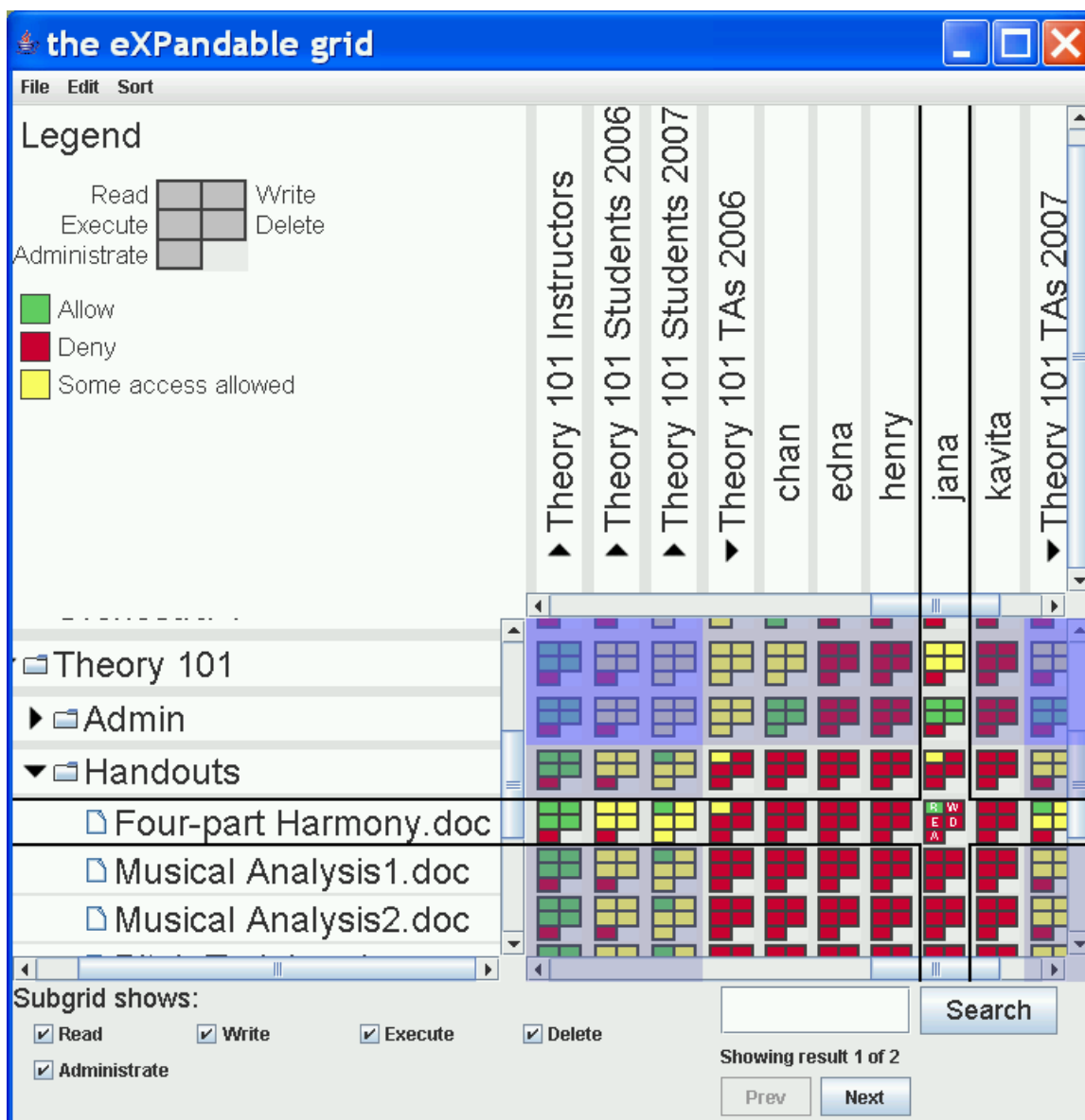
Figure 6.1: Screenshot of our Expandable Grid interface when the Jana task has been half-completed.
