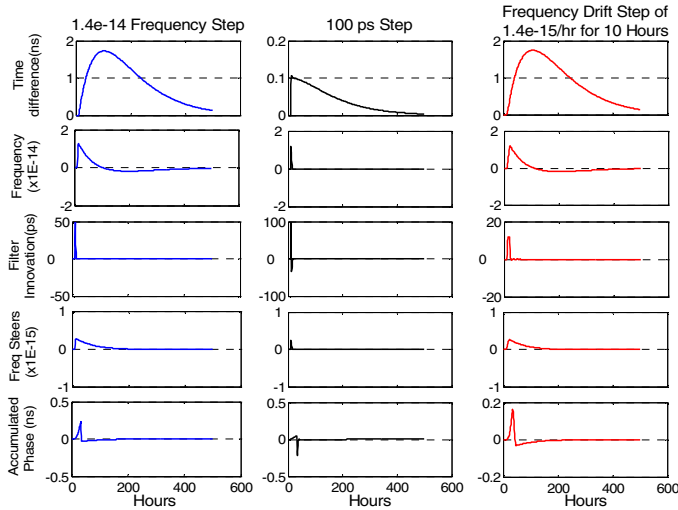
Figure 2. Shows the minimum frequency, phase, and drift steps that will cause the 2.7 \times 10^{-16} steer limit to be reached in the present system design.
