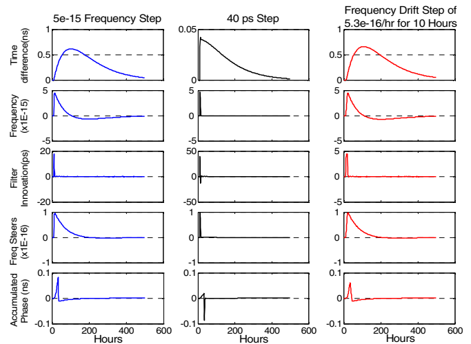
Figure 5. Shows the minimum frequency, phase, and drift steps that will cause the 1 \times 10^{-16} steer limit to be reached in the proposed system redesign.
