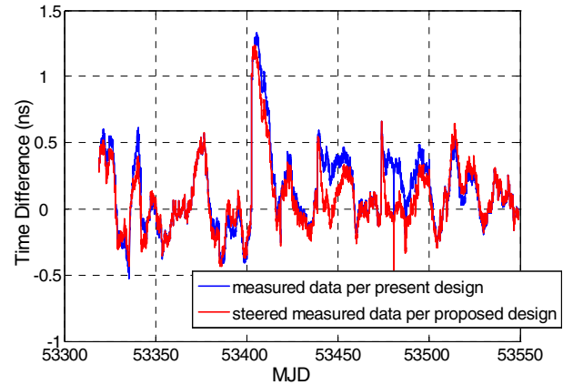
Figure 6. Time Difference of the Master Clock vs. USNO timescale as measured during operations and re-steered in simulation with the proposed 1\text{E-}16 steering limit.
