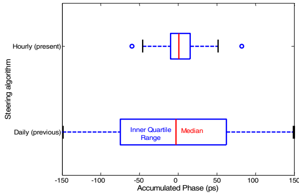
Figure 3. Box plot of daily accumulated phase of the previous and present control system designs.
