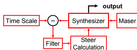
Figure 1. Block diagram of a typical control system that creates a physical realization of a timescale.
