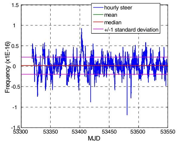
Figure 4. Frequency steers of the operational USNO Master Clock.
