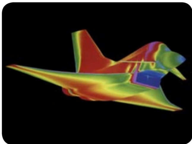
Computational fluid dynamics in Typhoon drag coefficient modelling.
