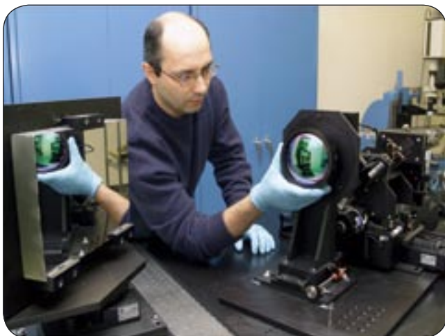
Optics lab measuring MTF of an infrared lens © BAE Systems.
