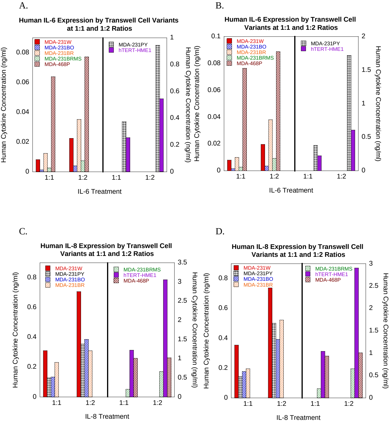
Figure 18.: Human Transwell Cell Variant Cytokine Response to Treatment with Murine MC3T3-E1 Osteoblasts 1:1 and 1:2 in a Transwell System.
