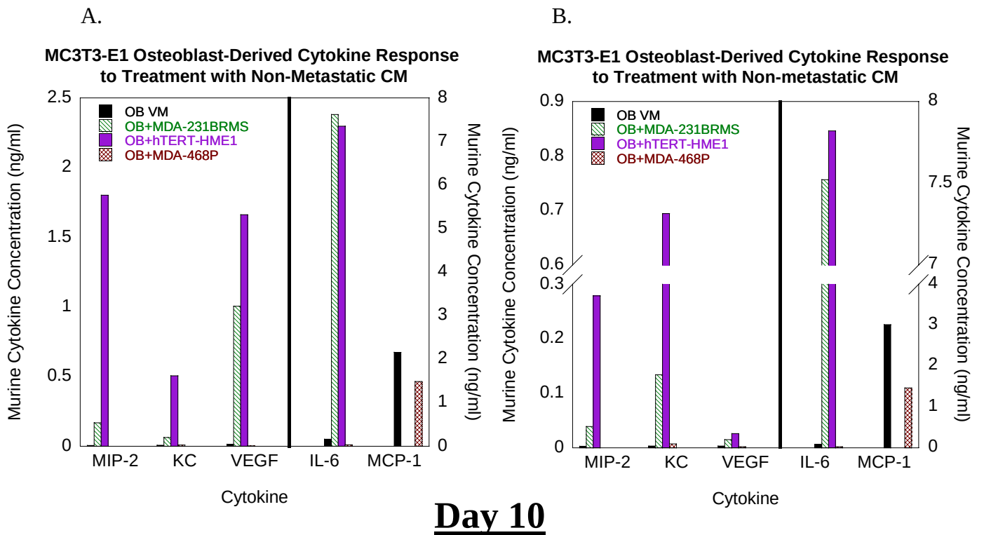
Figure 9.: Murine MC3T3-E1 cytokine response to treatment with 0 (VM) or 50% conditioned medium from human non-metastatic cell variants.
