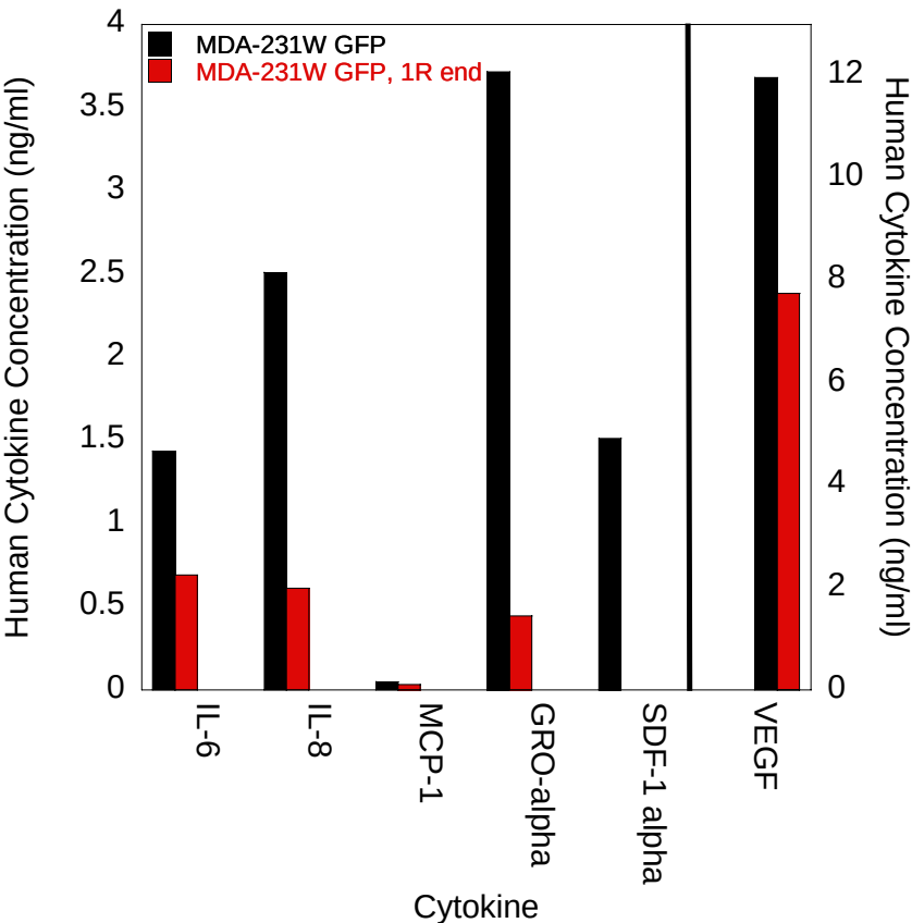
Figure 24.: The Human Cytokine Expression of Retrieved Intracardiac Inoculated Human Metastatic Breast Cancer Cell GFP Variants.
