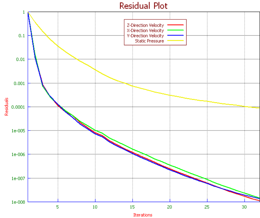
Figure 113. Residual Plot (Random Time, What Residuals Should Look Like)
