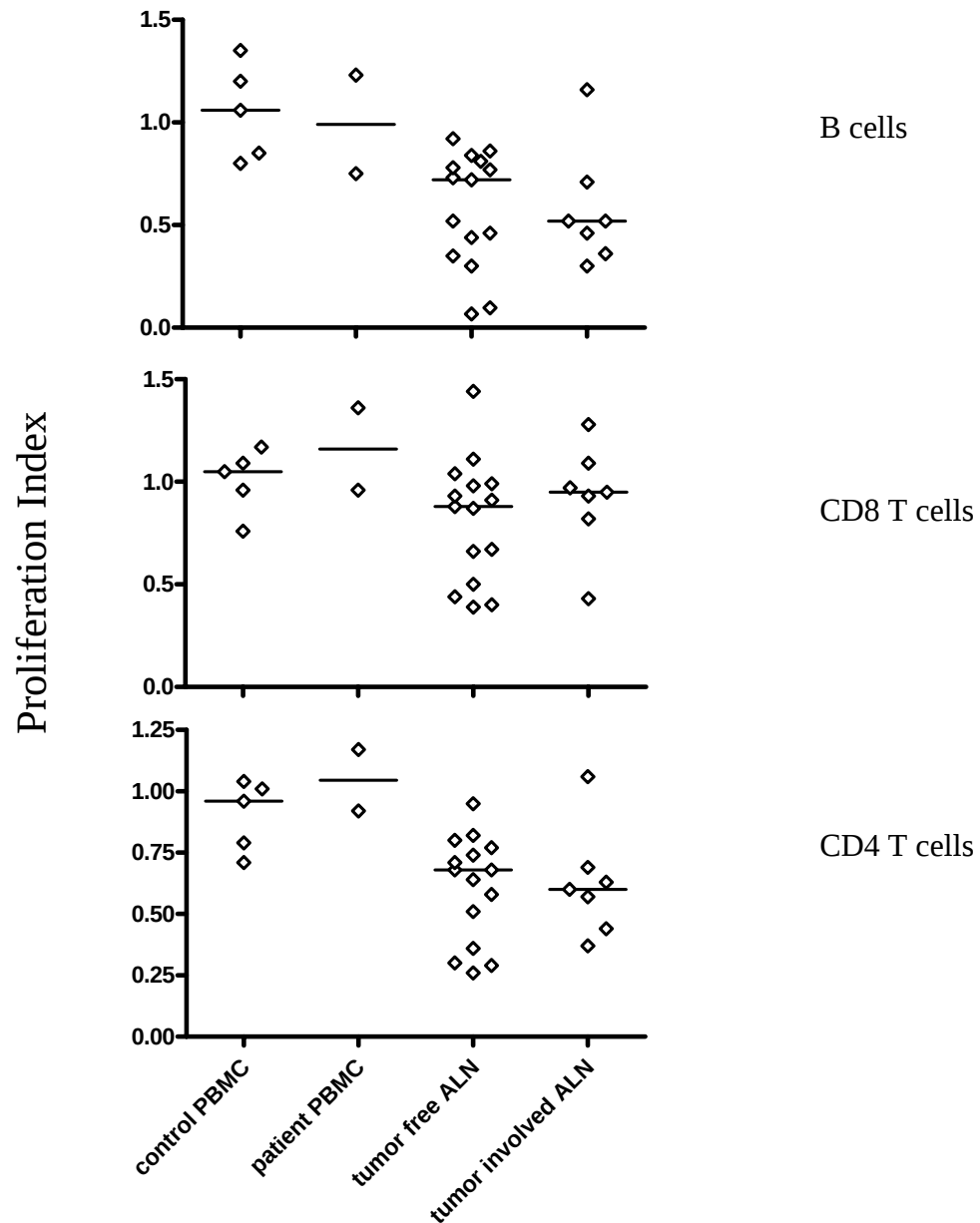
Figure A1. Isolated immune cells were labeled with CFSE and stimulated with phorbol esters/Ionomycin for 115hour. Cell divisions were analyzed by FACS Aria and cell proliferation analysis was performed by flowjo. Proliferation capability of B cells, CD8 T cells, CD4 T cells for 5 healthy control blood samples, 2 patient blood samples, 16 tumor free lymph nodes, 7 tumor involving lymph nodes are illustrated in separate scatter columns. Y axis indicates division index, the average number of divisions a cell has undergone. Medians are indicated by the bar in each scatter column.
