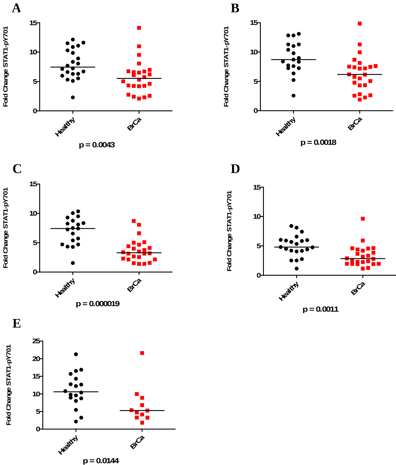
Figure A4. IFN- \alpha -Stimulated fold change in STAT1-pY701 in PBMC subsets from healthy ( ● ) and breast cancer patients (BrCa ■ ) with corresponding p-values as measured by Phosflow. PBMC subsets were gated based on surface markers measured by FACS. A: Lymphocytes, B: CD3 T cells, C: CD19 B cells, D: CD16 Natural Killer cells, and E: T regulatory cells.
