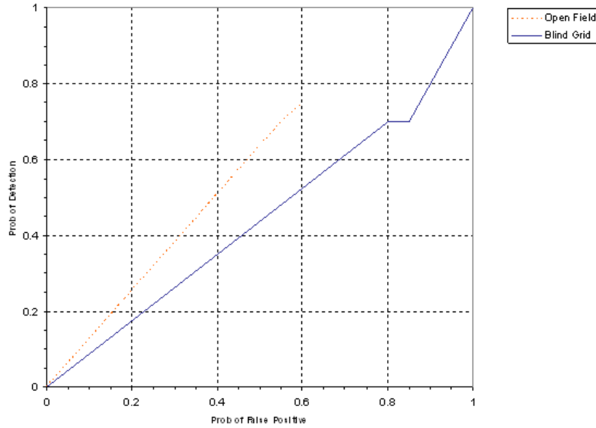
Figure 9. EM AMOS/towed P_d^{\text{disc}} versus the respective P_{fp} for ordnance larger than 20 mm.
