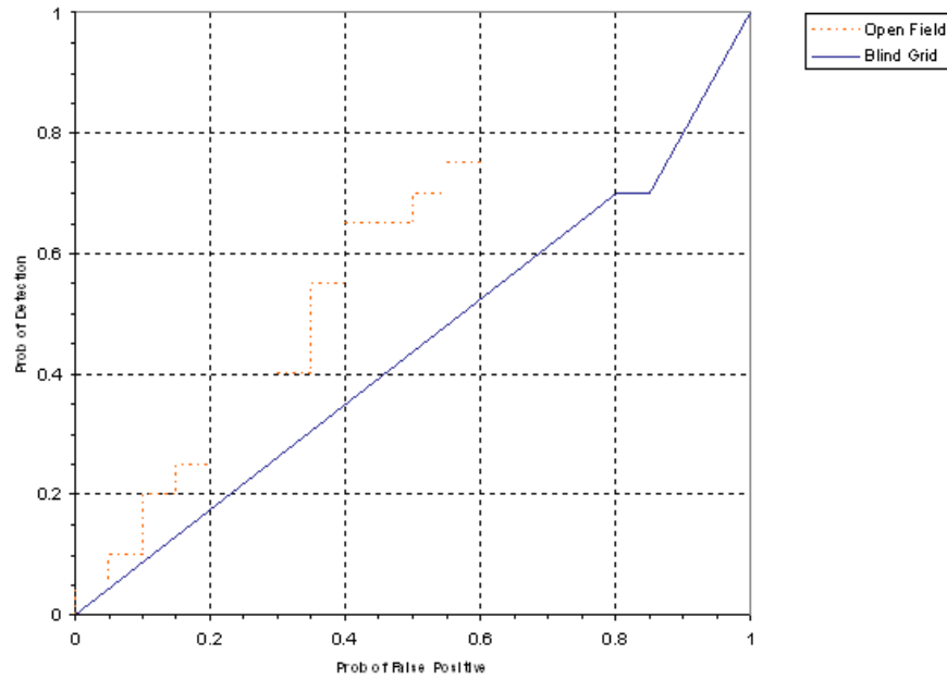
Figure 8. EM AMOS/towed P_d^{\text{res}} versus the respective P_{fp} for ordnance larger than 20 mm.
