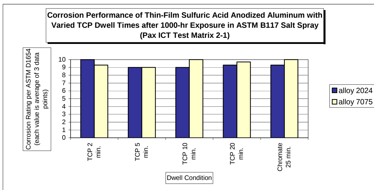
Figure 2: Corrosion Performance of TFSA Aluminum with Varied TCP Dwell Times after 1,000-hr Exposure in ASTM B 117 Salt Spray
