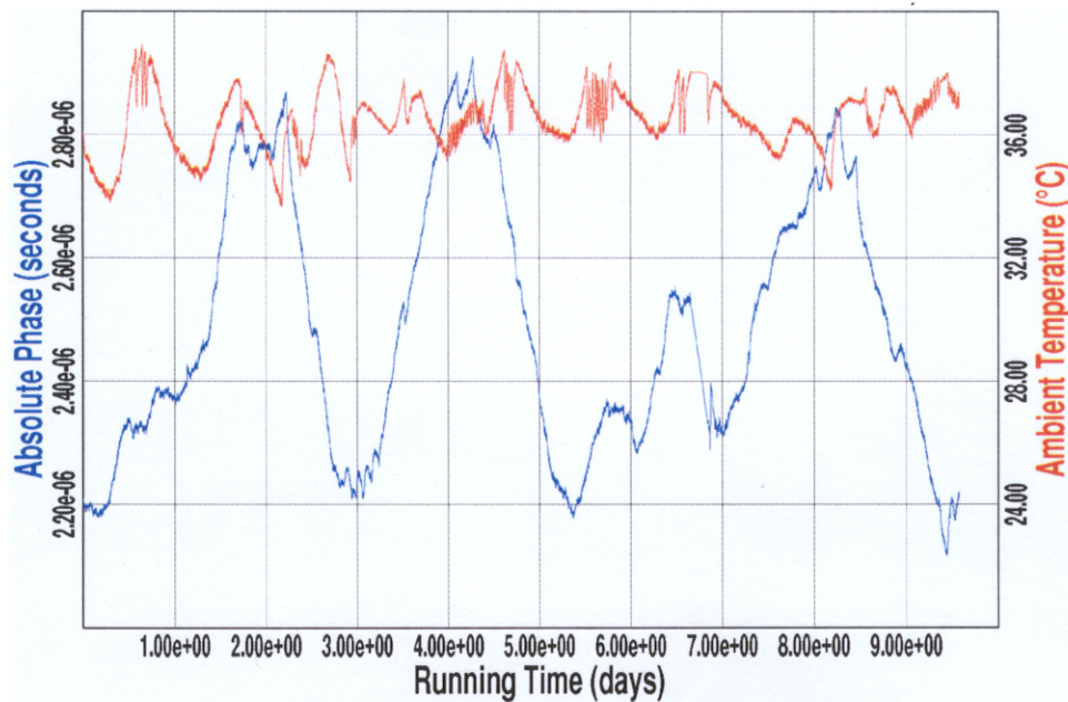
Figure 5 - CDMA 1PPS vs. GPS 1PPS Phase 14-24 Nov. 2001
