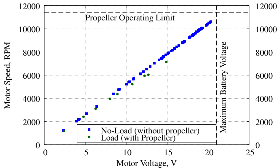
Figure 7.3: No-load motor speed
