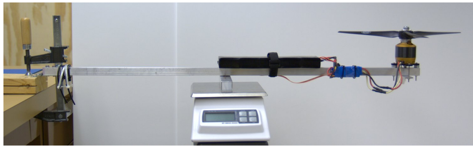
Figure 7.1: Single motor test fixture
