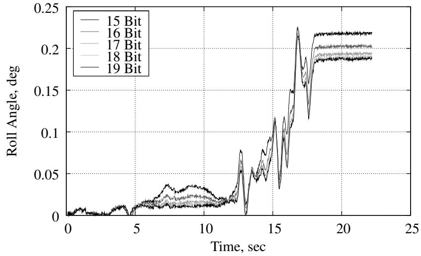
Figure 6.4: Roll Angle Error with Varying Mantissa Length
