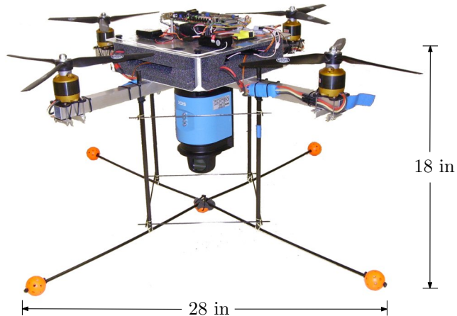
Figure 1.2: AEC quadrotor
