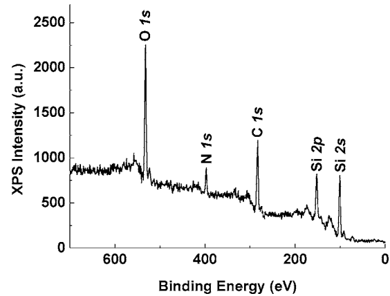
FIG. 2. XPS survey scan for a 1800 °C/15 s microwave-annealed virgin 4H-SiC sample.
