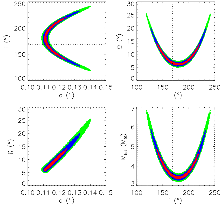
Figure 5. Crosscuts through the \chi^2 surfaces derived from the fit to the HST measurements alone while holding the spectroscopic parameters fixed. These results were obtained by performing a Monte Carlo search for orbital solutions within the 3\sigma confidence interval ( \Delta\chi^2 = 9 ). The total mass was derived for each of the 10,000 orbits found within this interval using a parallax of 7.72 mas. The dotted lines indicate the critical value of the inclination ( i = 168^\circ ), above which negative values of a component mass are produced. The color codes in the electronic version of this figure correspond to the 1\sigma (red), 2\sigma (blue), and 3\sigma (green) confidence intervals.
