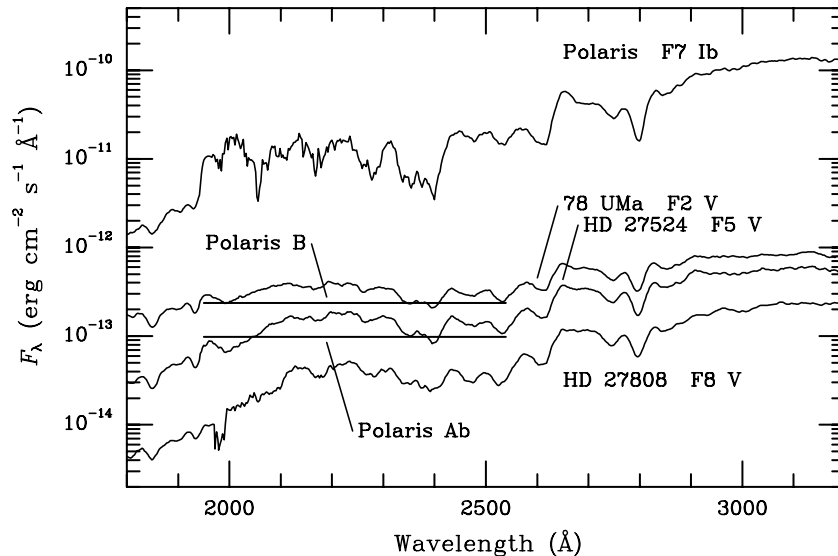
Figure 11. IUE UV spectra of Polaris and of three main-sequence F-type stars scaled to the distance of Polaris using the respective Hipparcos parallaxes. The two horizontal lines correspond to the mean flux levels in the F220W filter of the ACS/HRC of Polaris B (top) and Ab (bottom). The lengths of the horizontal lines correspond to the FWHM of the filter. On the basis of its UV flux level, Polaris B is inferred to have a spectral type near F3-F4 V, in good agreement with its ground-based classification at F3 V. Polaris Ab is inferred from its F220W flux to have a spectral type near F6 V.
