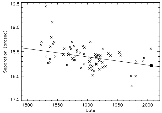
Figure 10. Separation measurements of Polaris B relative to Polaris A. Our HST measurements are marked by the two filled circles. The solid line shows a linear least-squares fit yielding a rate of change in the separation of -1.67 \pm 0.19 \text{ mas yr}^{-1} .
