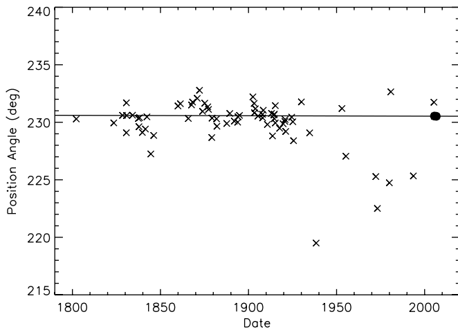
Figure 9. Historical measurements of the position angle of Polaris B relative to Polaris A, precessed to the equinox of J2000.0. Our HST measurements are marked by the two filled circles. The solid line shows a least-squares fit yielding a rate of change in the position angle of -0^{\circ}.00035 \pm 0^{\circ}.00094 \text{ yr}^{-1} .
