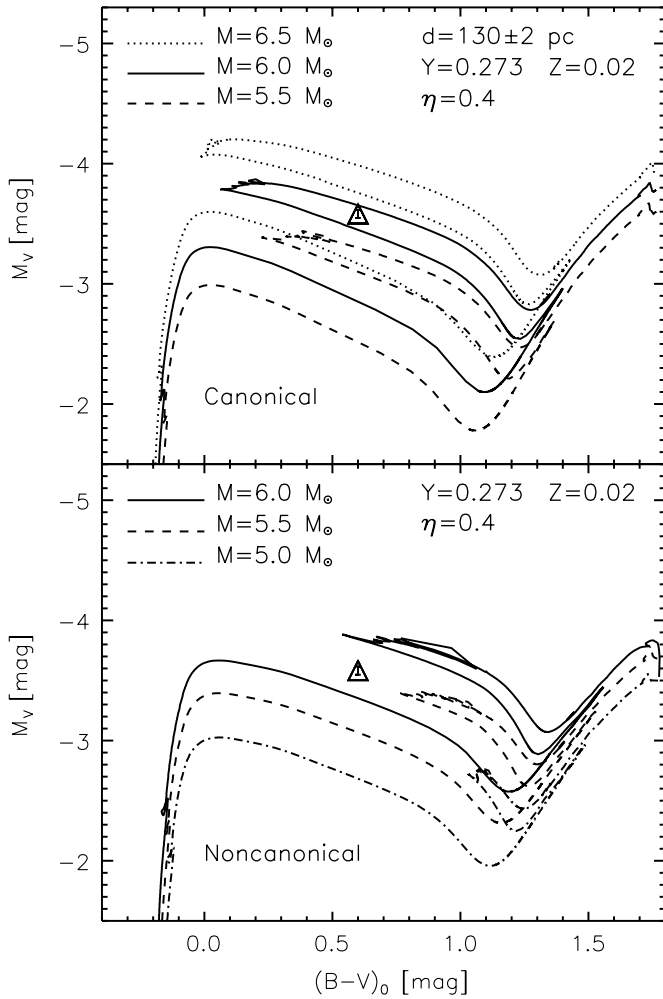
Figure 12. Evolutionary tracks (see Pietrinferni et al. 2006) in the M_V vs. (B - V)_0 plane, with the location of Polaris marked (open triangle enclosing error bar). Top panel: canonical evolutionary models neglecting convective core overshooting during H-burning phases. Bottom panel: noncanonical evolutionary models including convective core overshooting. The assumed Polaris distance and helium ( Y ) and metal ( Z ) abundances (scaled solar) are indicated in the figure, and the legends on the left indicate the stellar masses for each track. These models include mass loss with a Reimers parameter \eta = 0.4 .
