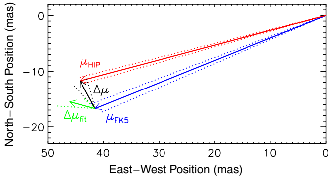
Figure 7. Schematic comparison between the instantaneous and mean proper motions of Polaris A. The vectors indicate the magnitude and direction of the annual proper-motion measurements from Hipparcos ( \mu_{\text{HIP}} ; red), the long-term average FK5 ground-based motion ( \mu_{\text{FK5}} ; blue), and the vector difference between the two ( \Delta\mu ; black). Dotted red and blue lines indicate the 1\sigma uncertainties in the Hipparcos and FK5 measurements. The green vector represents the best fit difference between the proper motions ( \Delta\mu_{\text{fit}} ) computed from our simultaneous orbit fit to the HST measurements and the proper-motion data while holding the spectroscopic parameters fixed (see Section 3.3).
