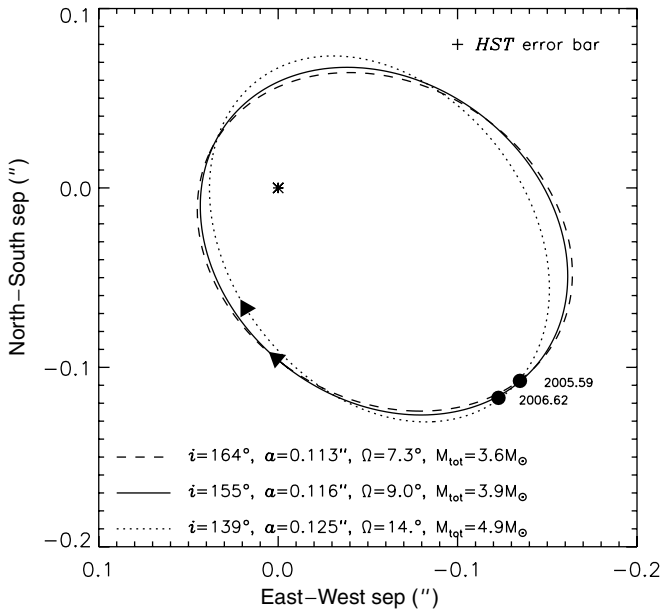
Figure 6. Three examples of orbits resulting from variations of the orbital parameters within the 1\sigma confidence intervals based on the fit to the HST measurements alone while holding the spectroscopic parameters fixed. The arrows indicate the direction of motion. All three orbits fit the HST measurements (filled circles) within the 1\sigma error bar shown at the top of the figure, but they imply total system masses ranging from 3.6 to 4.9 M_\odot .
