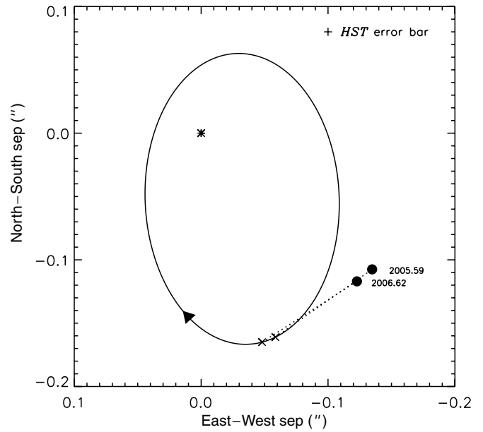
Figure 4. Comparison of the retrograde orbital solution of Wielen et al. (2000; solid ellipse) with our HST measurements of Polaris Ab (filled circles). The arrow indicates the direction of motion. The orbit was calculated by fixing the spectroscopic and astrometric orbital parameters (see Table 3) and solving only for the semimajor axis based on the HST separation measurements. We found a = 0''.131 . The dotted lines connect the observed positions to \times symbols marking the predicted positions, and show the inadequacy of this simple solution at predicting the P.A.s. The size of the HST error bar is indicated by the cross at the top of the plot.
