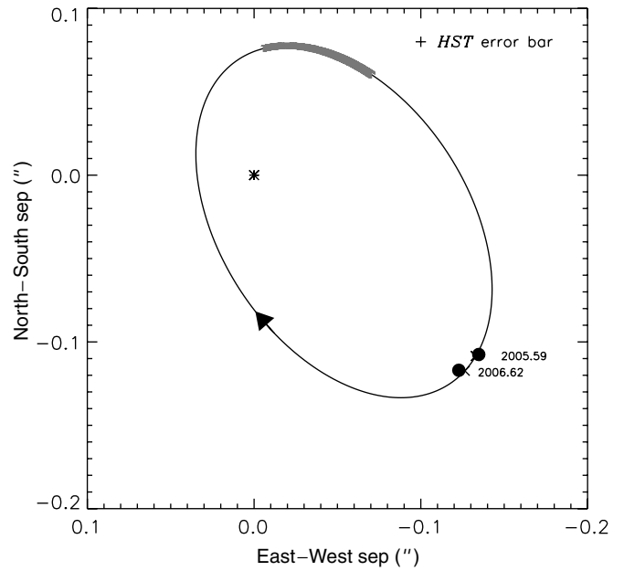
Figure 8. Final best fit orbit of Polaris Ab relative to Aa based on a simultaneous fit to the HST measurements (filled circles) and the proper-motion data while holding the spectroscopic parameters fixed. The predicted orbital positions at the epochs of the HST measurements are marked by the \times symbols (partially hidden by the observed points). The position of the companion during the time frame of the Hipparcos mission is highlighted by the shaded gray line segment; its direction of motion is of course 180^\circ different from the direction of \Delta\mu_{\text{fit}} , shown as a green arrow in Figure 7.
