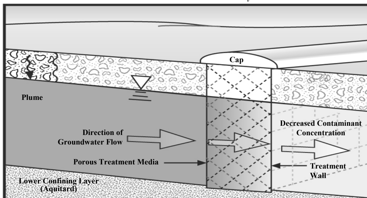
Model of a Permeable Reactive Barrier System
