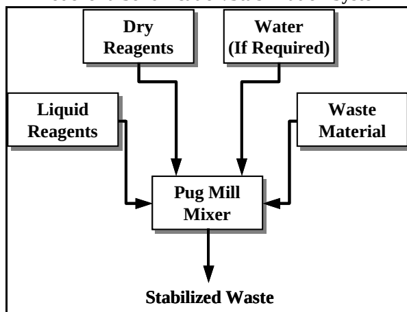
Model of a Solidification/Stabilization System
