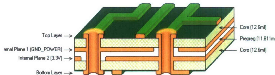
Figure 3.3: New interface board PCB layer stack
