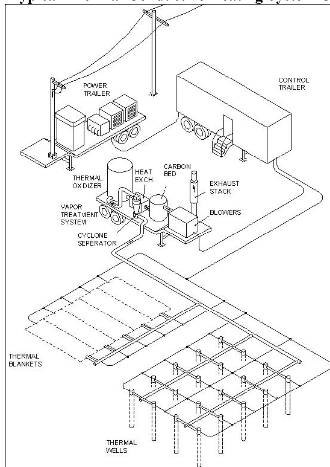
Figure 3-3: Typical Thermal Conductive Heating System Configuration
