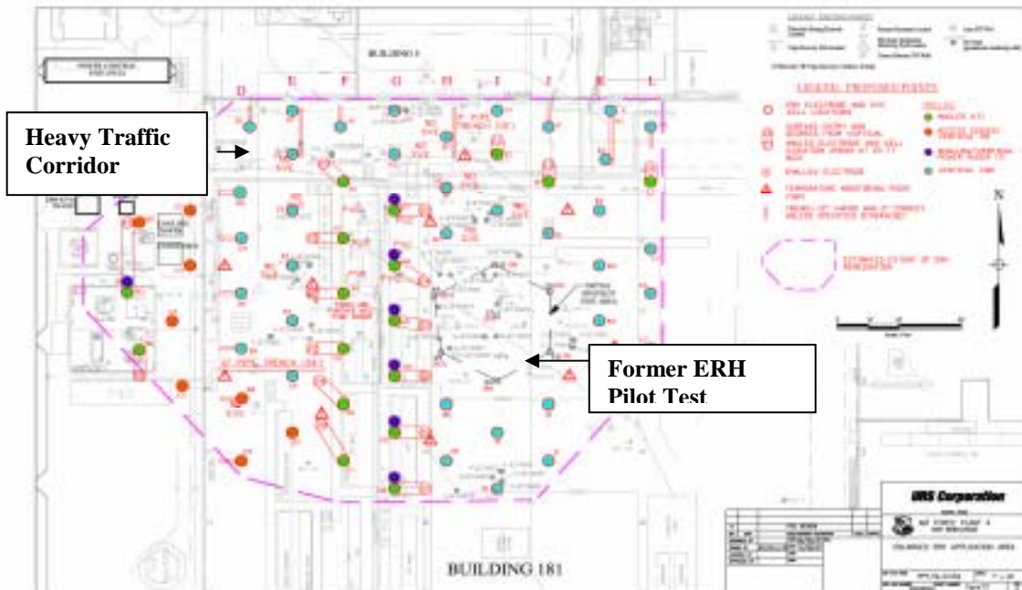
Figure 1. ERH System Layout Inside Building 181
