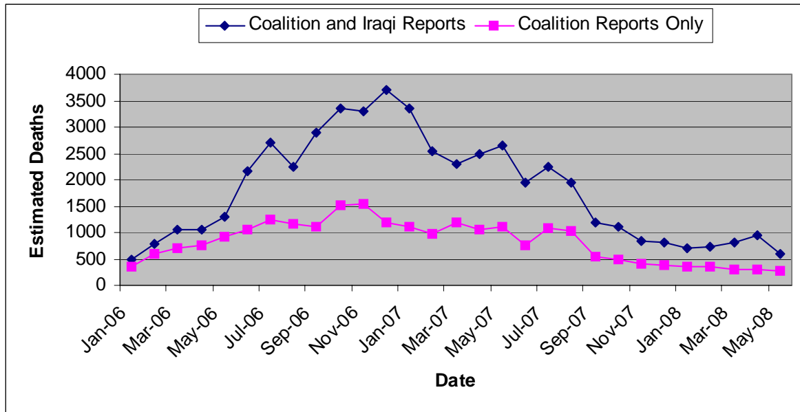
Figure 1. Estimated Iraqi Civilian Deaths, January 2006 to May 2008
