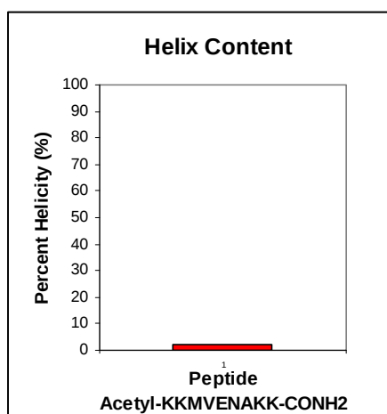
Figure 9. AGADIR™ predicted helicity of the peptide KKMVENAKK.
