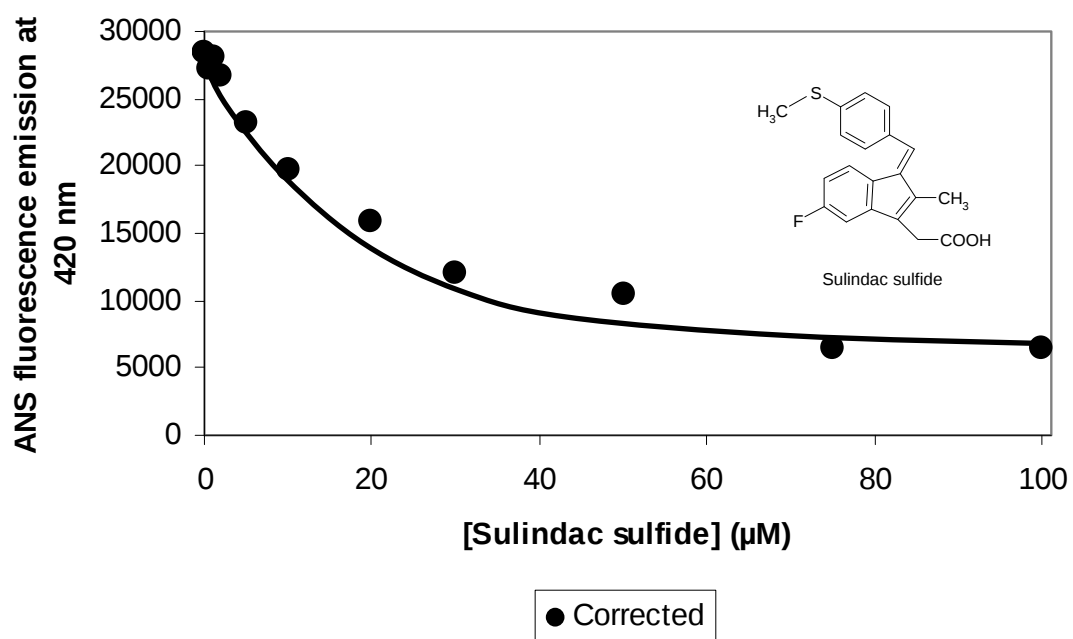
Figure 18.8. Corrected saturation binding curve experiment of MsrA with sulindac sulfide. [ANS] = 15 μM.
