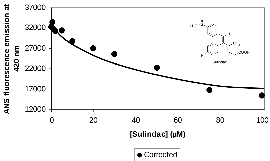
Figure 18.9. Corrected saturation binding curve experiment of MsrA with sulindac. [ANS] = 15 μM.
