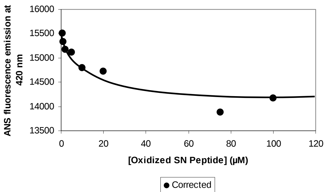
Figure 17.6. Corrected saturation binding curve of MsrA with oxidized SN peptide. [ANS] = 300 μM.
