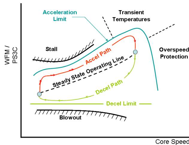
Figure 1. Transient Operability
