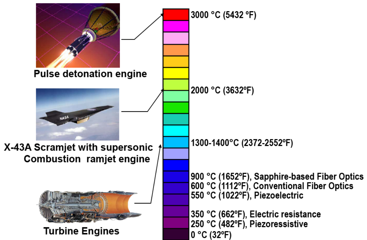
Figure 1. High Temperature Regimes for Sensors with Aerospace applications.
