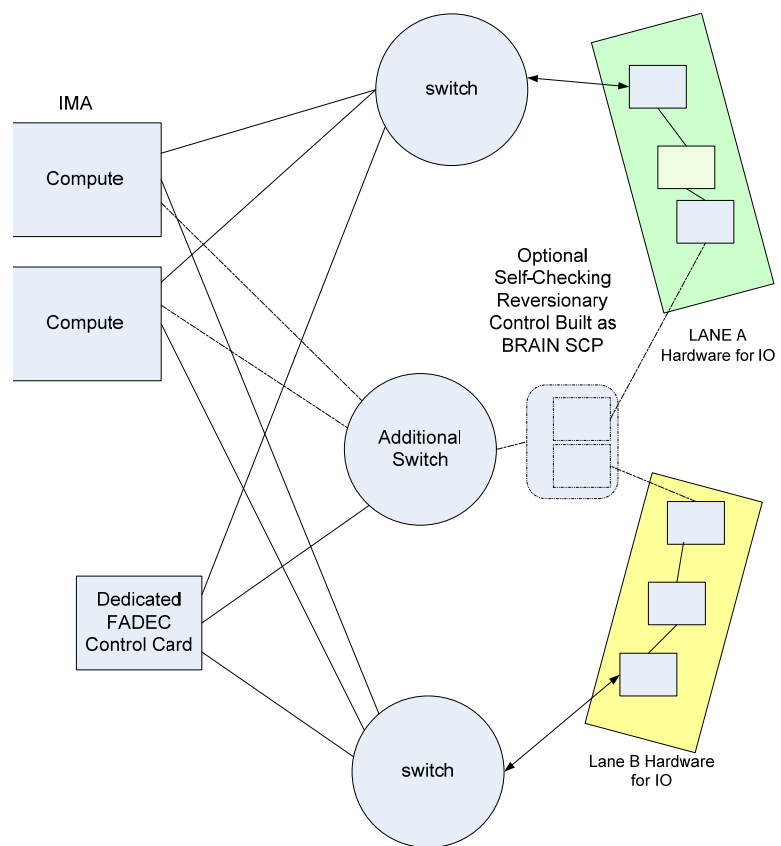
Figure 7. Architectural Options for Reversionary Backup control
