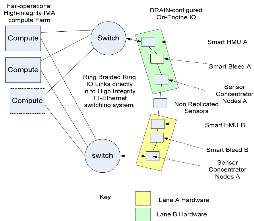
Figure 6. Architectural HW Lane mapping
