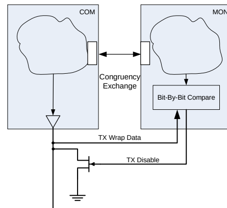
Figure 2. TTEthernet Command/Monitor Configuration
