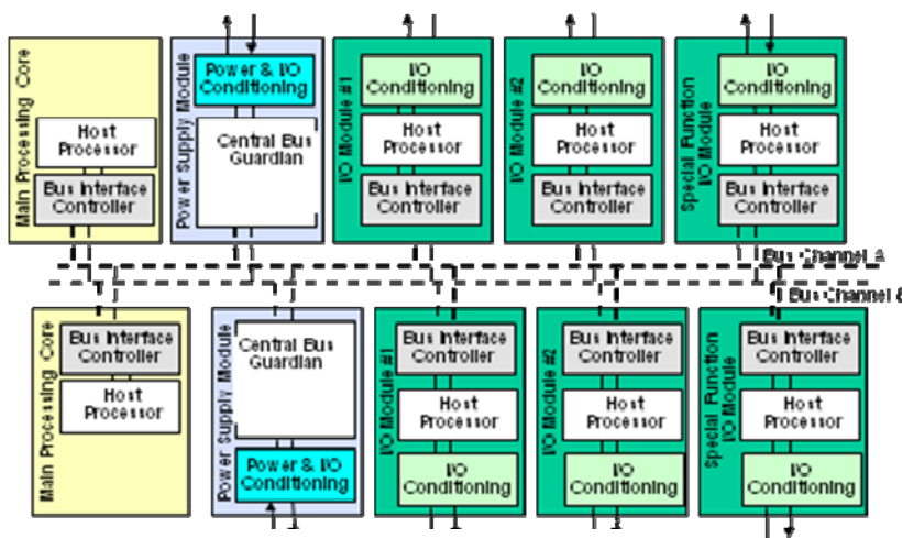
Figure 1: Generation 1 MAC Architecture
