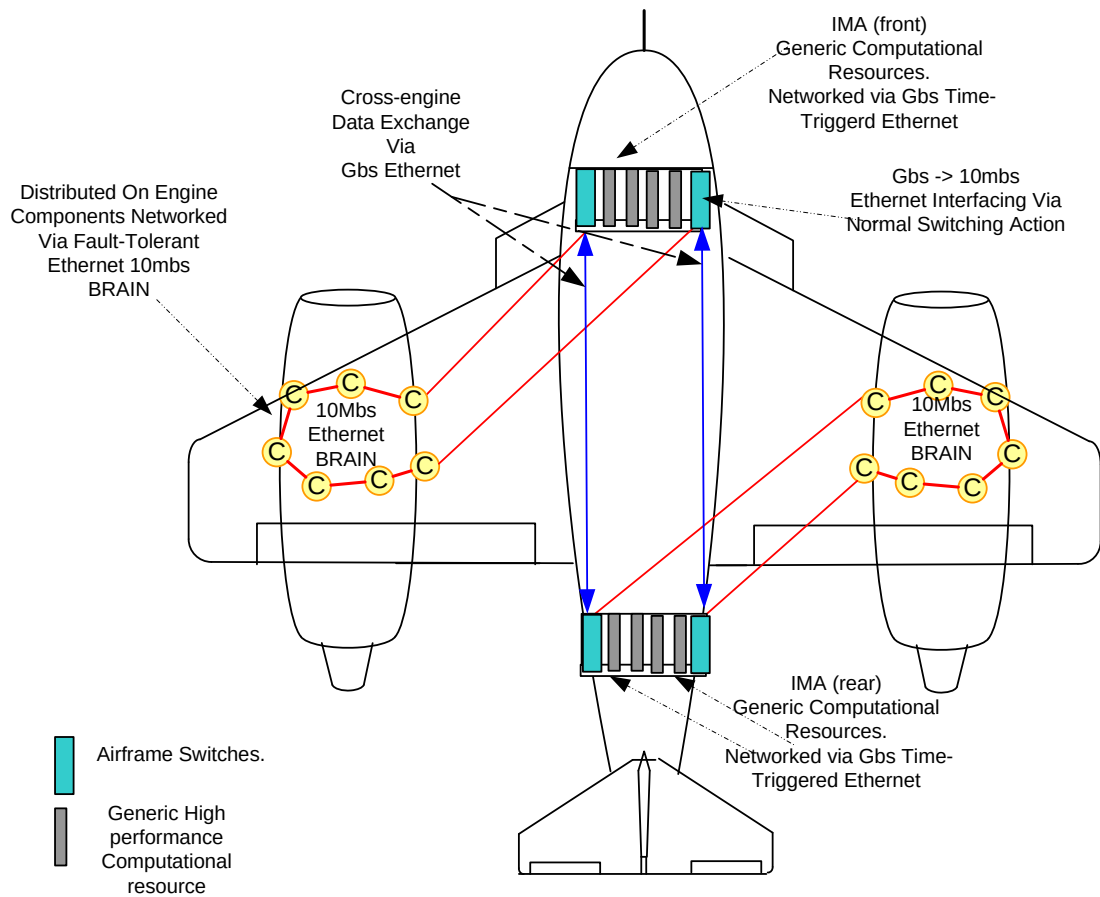
Figure 4. Hybrid BRAIN TTEthernet Architecture
