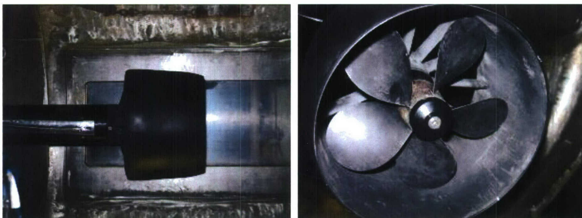
Figure 7. Ducted Configuration for Propeller 4381.
