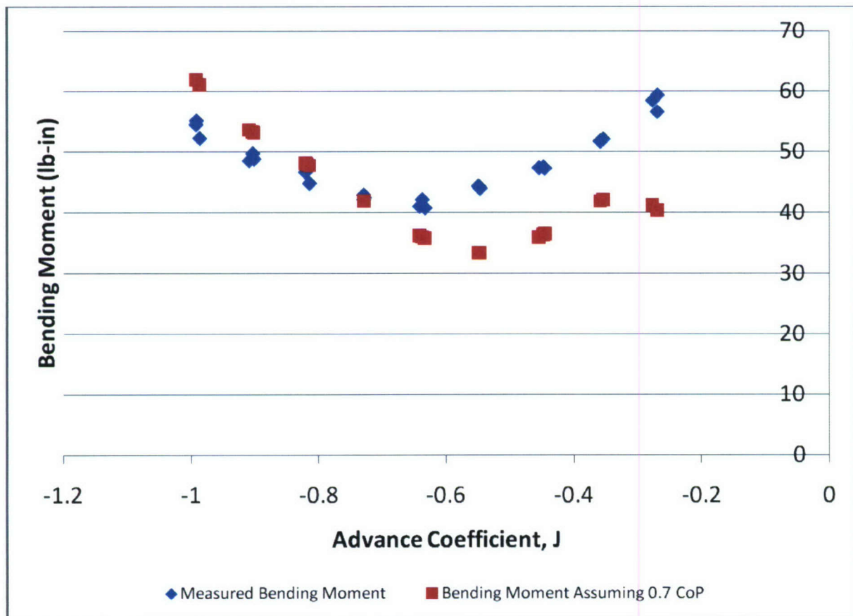
Figure 20. Bending moment calculated assuming a center of pressure of 0.7R .
