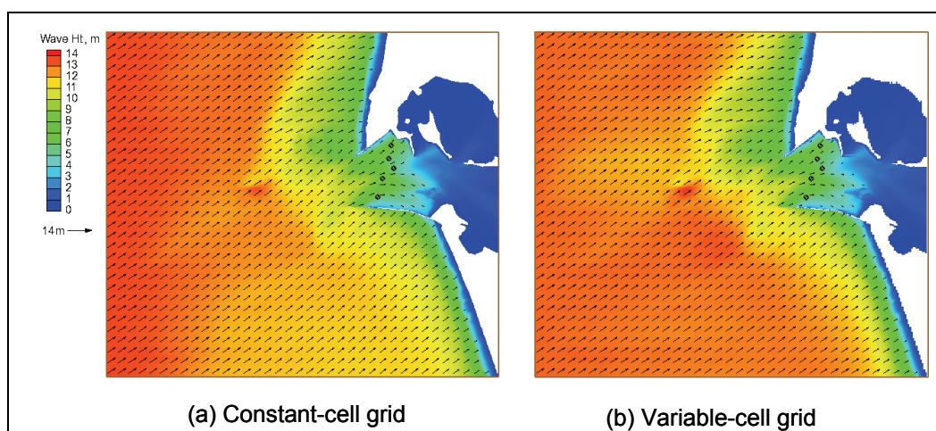
Figure 54. Calculated wave fields in fast mode, 13:00 GMT, 4 February 2006.
