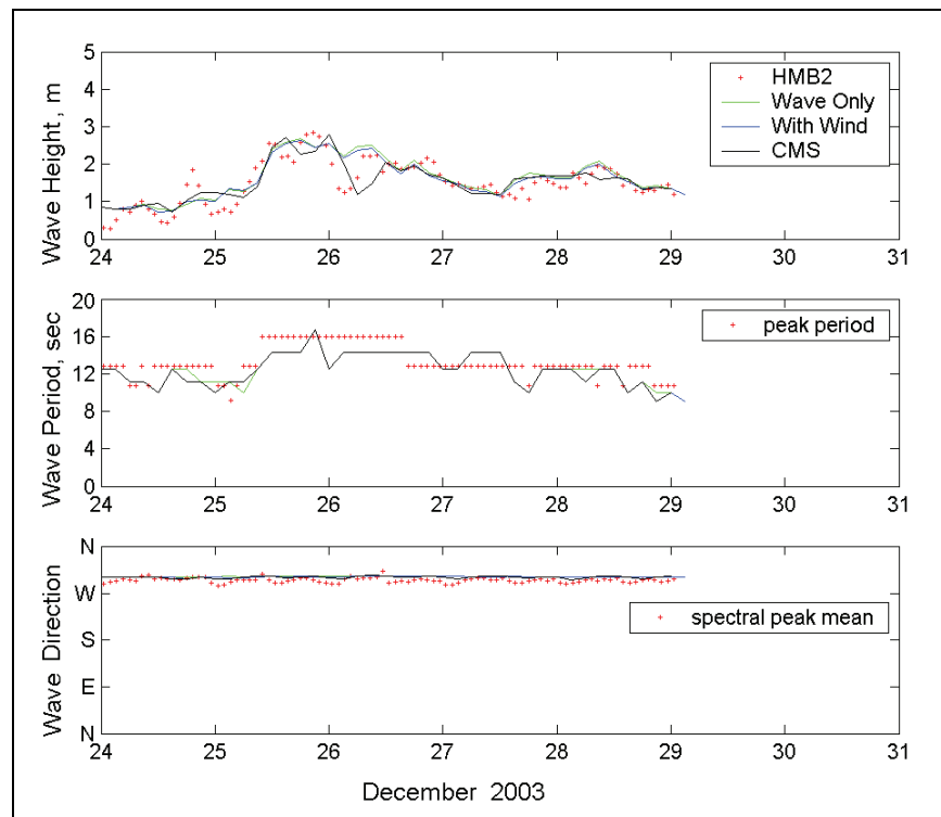
Figure 88. Measured and calculated waves at HMB02, 24-28 December 2003.
