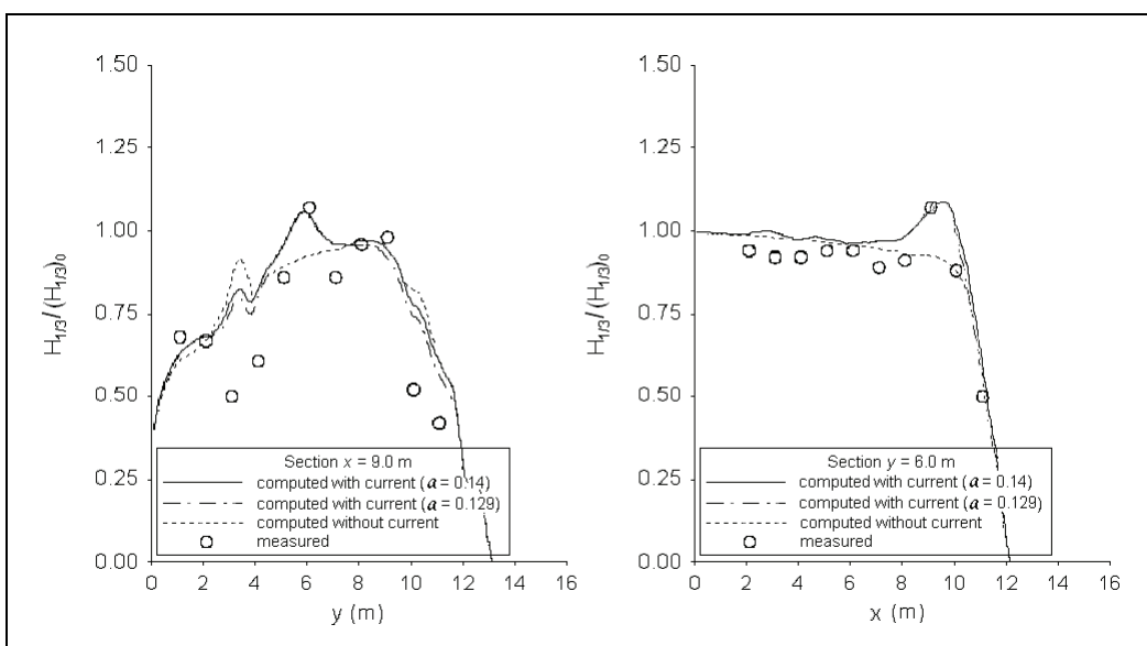
Figure 60. Normalized wave height comparisons of directional waves along longitudinal (left) and transverse (right) transects with the Extended Miche formula.
