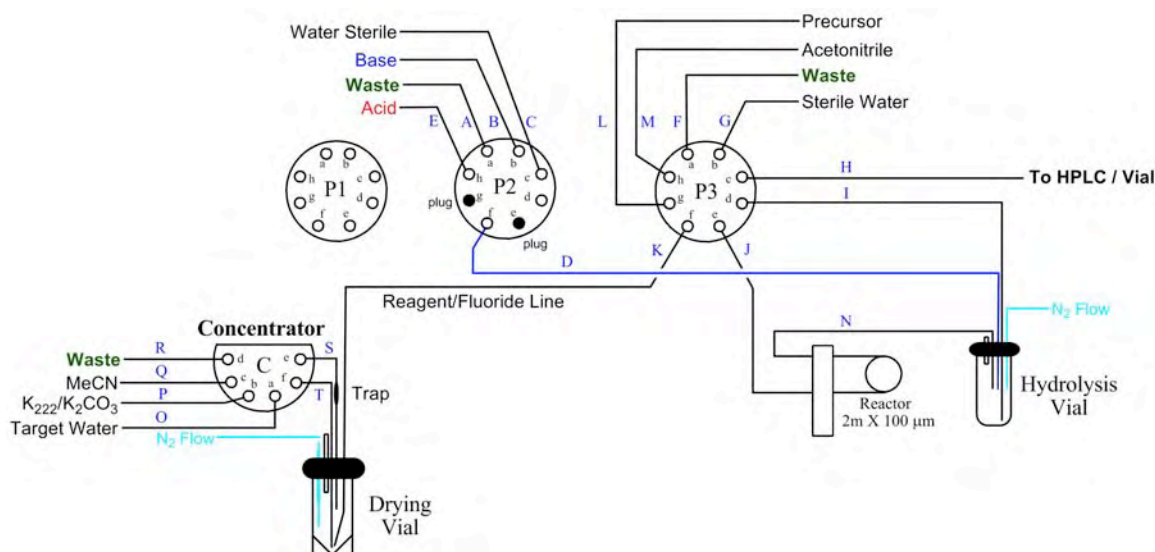
Figure 3: Batch plumbing diagram.
