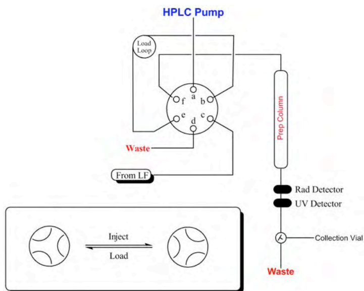
Figure 1: NanoTek LF to HPLC injector loop.
