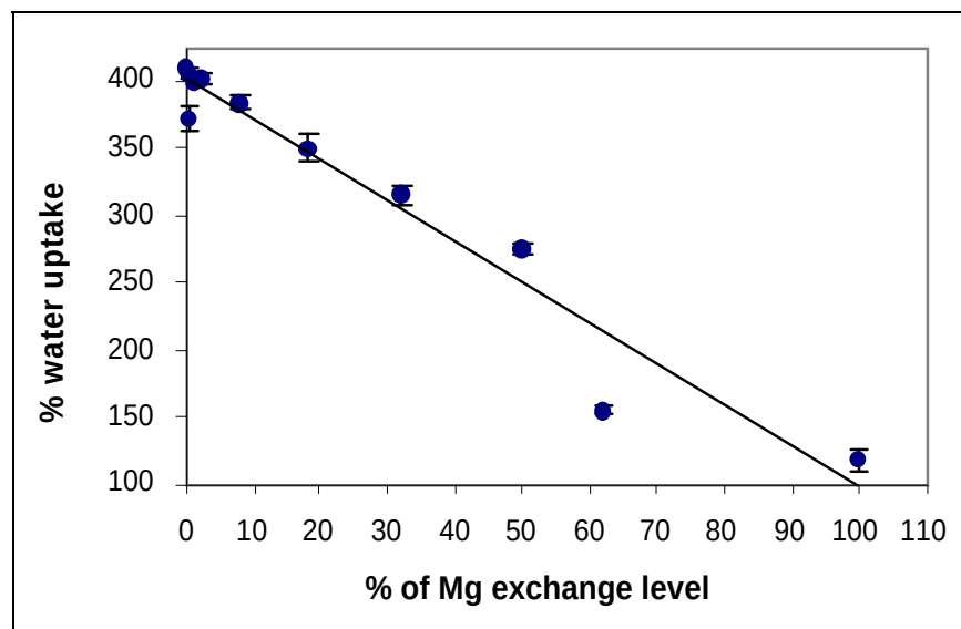
Figure 8. Correlation between water sorption and Mg exchange level.
