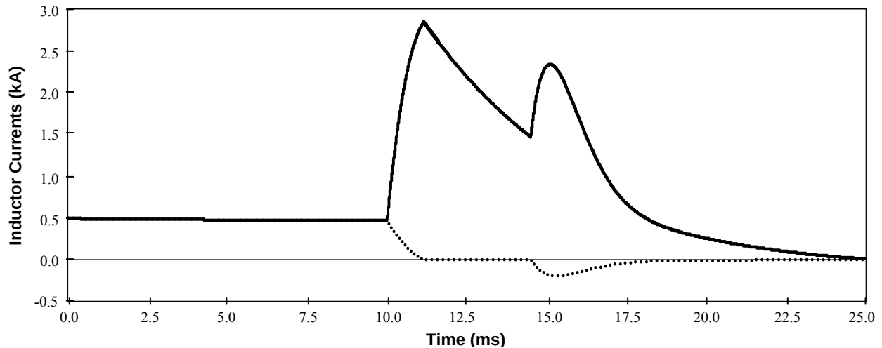
Figure 37: Inductor Currents in an Inductive Pulse Forming Network
