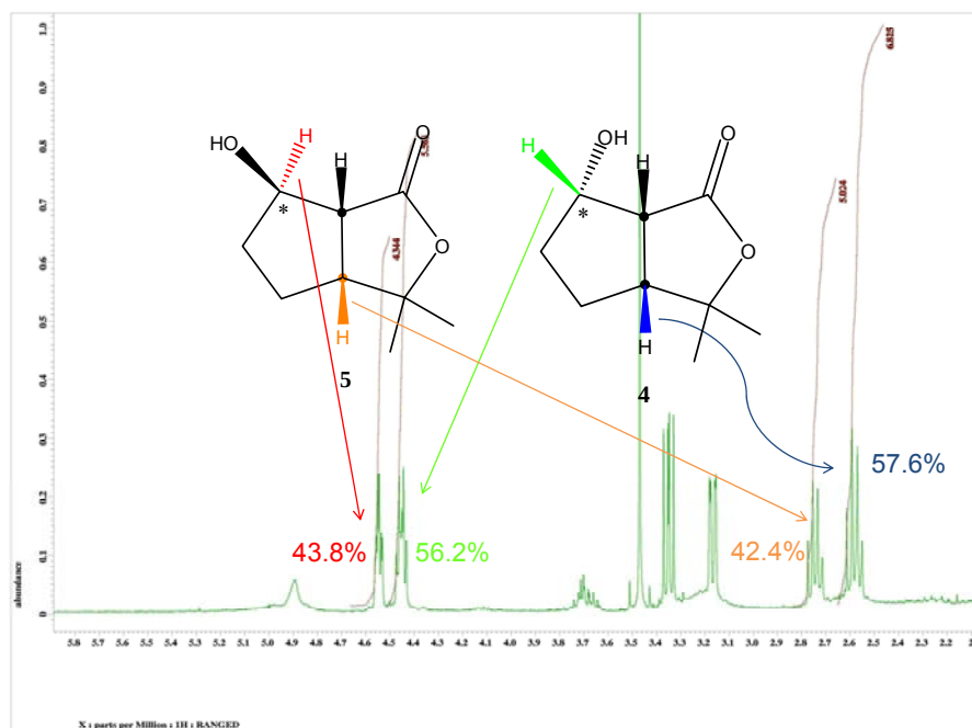
Figure 25: 1 H-NMR Spectrum Showing NaBH 4 Reduction Ratio @ 25°C
