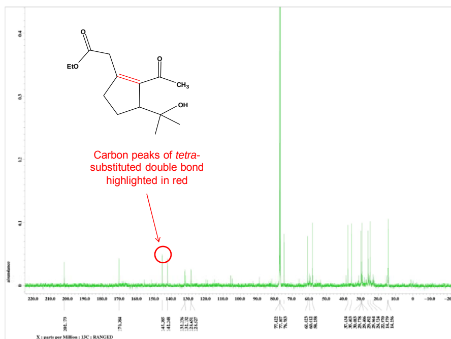
Figure 15: ^{13}\text{C} -NMR Spectrum Highlighting Tetra -substituted Carbon Double Bond Peaks
