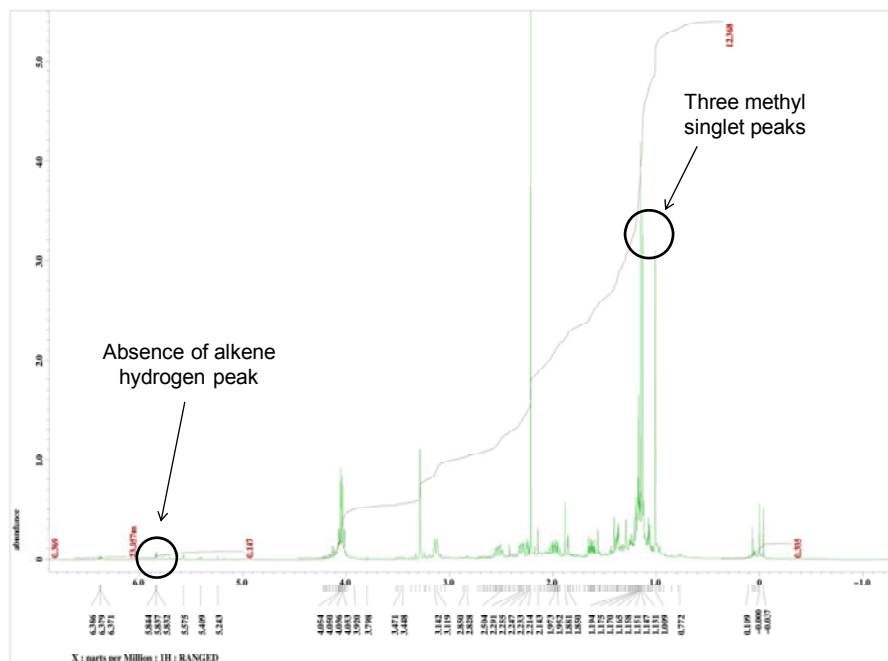
Figure 14: Disappearance of Double Bond Proton with New Methyl Peak
