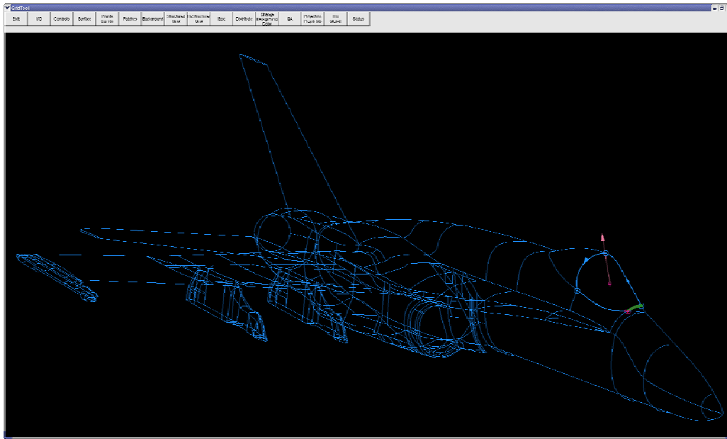
Figure 8. Surface patches used in model of F-18C
