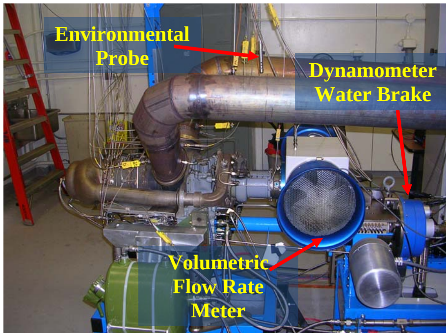
Figure 13 Other Instrumentation
