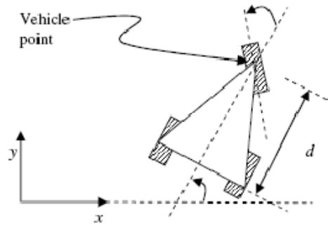
Figure 3: Non-holonomic vehicle.
