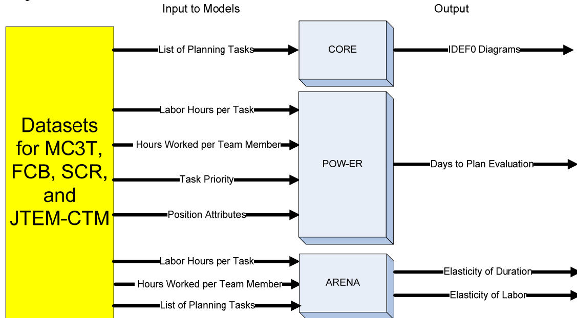
Figure 8: JC3M modeling overview
