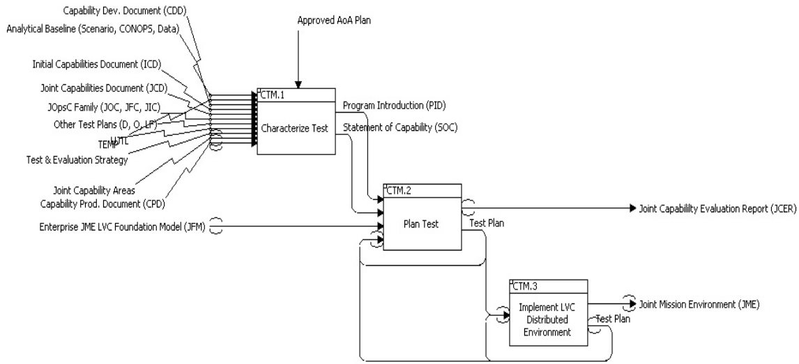
Figure 4: JTEM CTM in IDEF0
