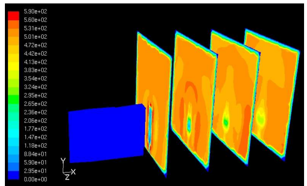
(b) Velocity magnitude (m/s): YZ planes ( 1.2 < d_e < 22.3 ).
