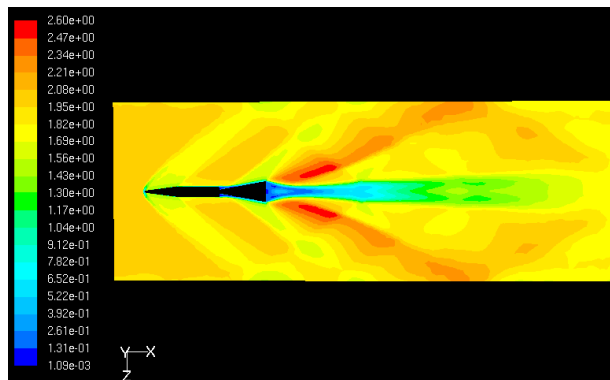
(a) Mach number: XZ plane ( y = 45 mm).
