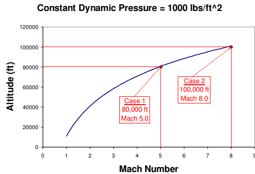
Figure 5. Dynamic pressure curve.
