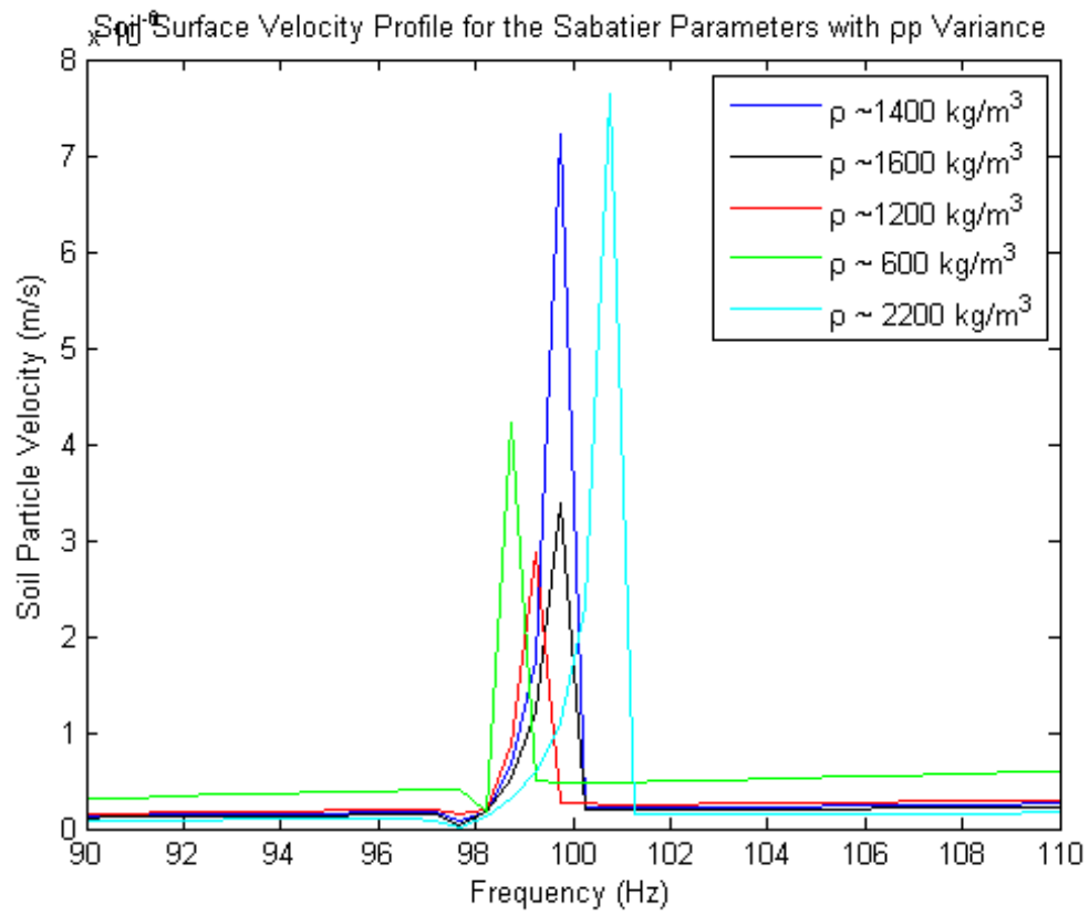
Figure 9.5: This graphic demonstrates the sensitivity of the soil particle velocity to changes in \rho_p . The vertical scale is 1 \times 10^{-6} .
