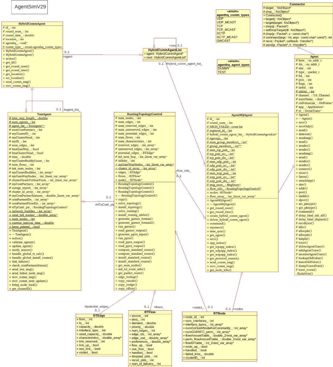
Figure 8. Class model for Llewellyn's fault-tolerant routing algorithm in ns2. AgentHQAgent provides the single interface to the ns2 simulation. This model is not easily extendable due to high coupling and low cohesion.
