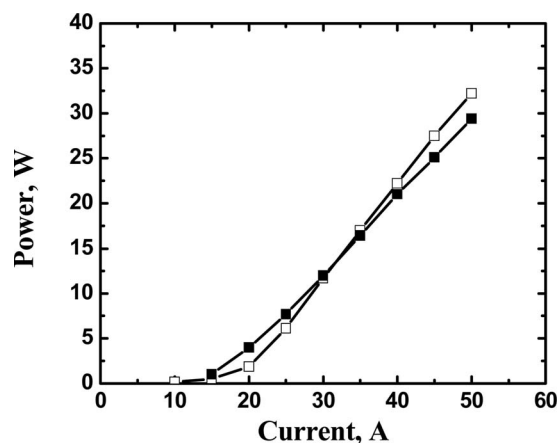
Fig. 3. cw output power of a free-running (empty square) and a volume Bragg (filled square) LDBs versus driving current.
