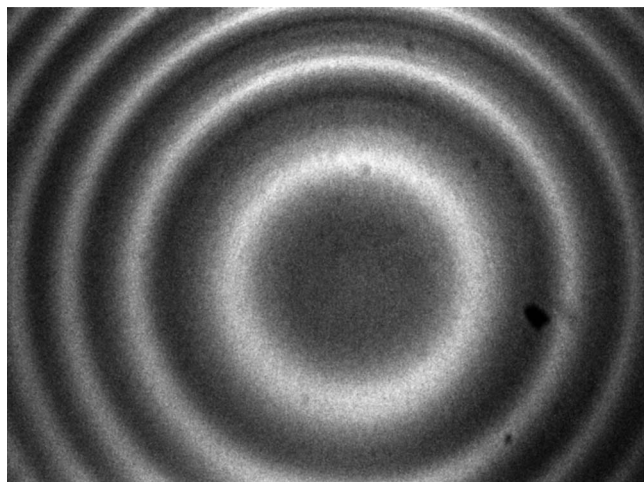
Fig. 2. Emission spectrum of the VOBLA measured using a Fabry–Perot interferometer with a 15 GHz FSR.
