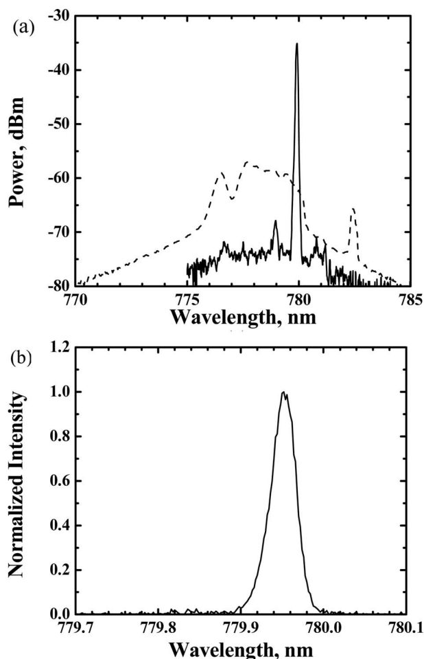
Fig. 1. (a) Emission spectra of free-running (dashed curve) and volume Bragg (solid curve) diode lasers in semi-log scale. (b) Emission spectrum of a VOBLA in linear scale.
