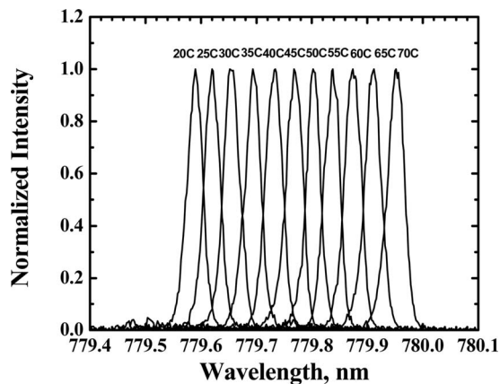
Fig. 4. Emission spectra of a volume Bragg diode laser at different grating temperatures.
