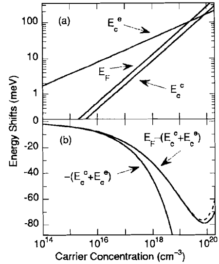
FIG. 2. (a) Predicted magnitudes of energy shifts due to E_F , E_c^* , and E_c^e in n -type ZnO, from Eqs. (3)–(5). (b) Decrease in energy gap with and without band filling for \alpha=0 (solid curves) and \alpha=0.502 (dashed curves).
