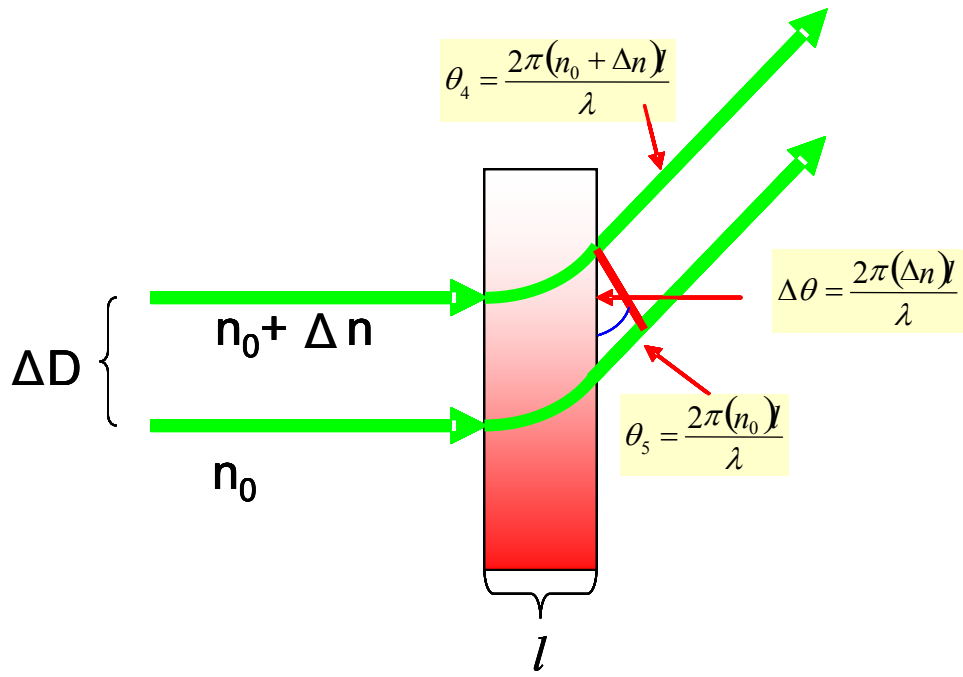
Graded index of refraction medium
