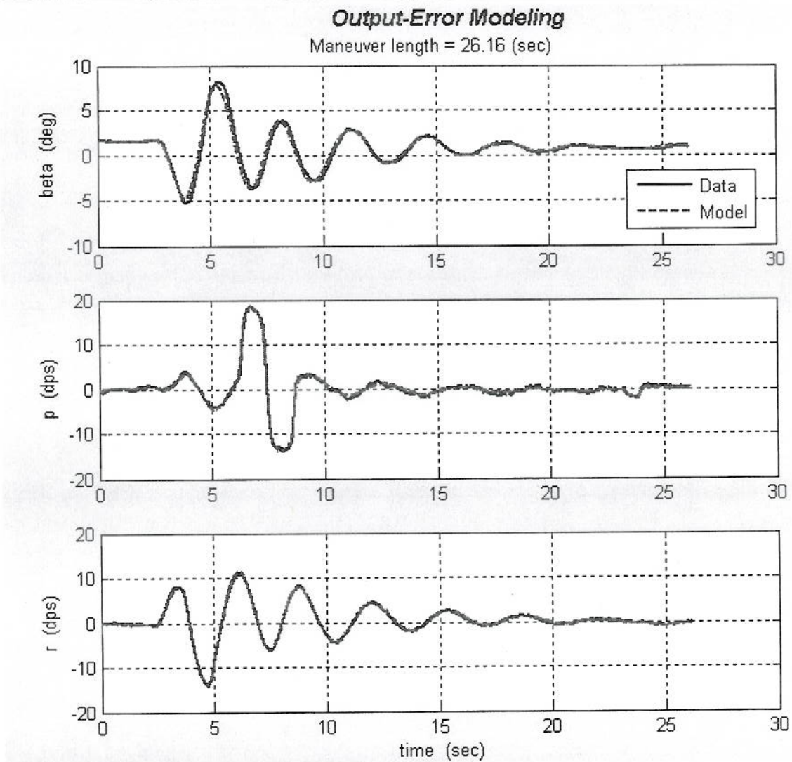
Figure E-6: Sample Results from a Yaw Roll Doublet (Wingtips On, Glide, 80 KIAS)
