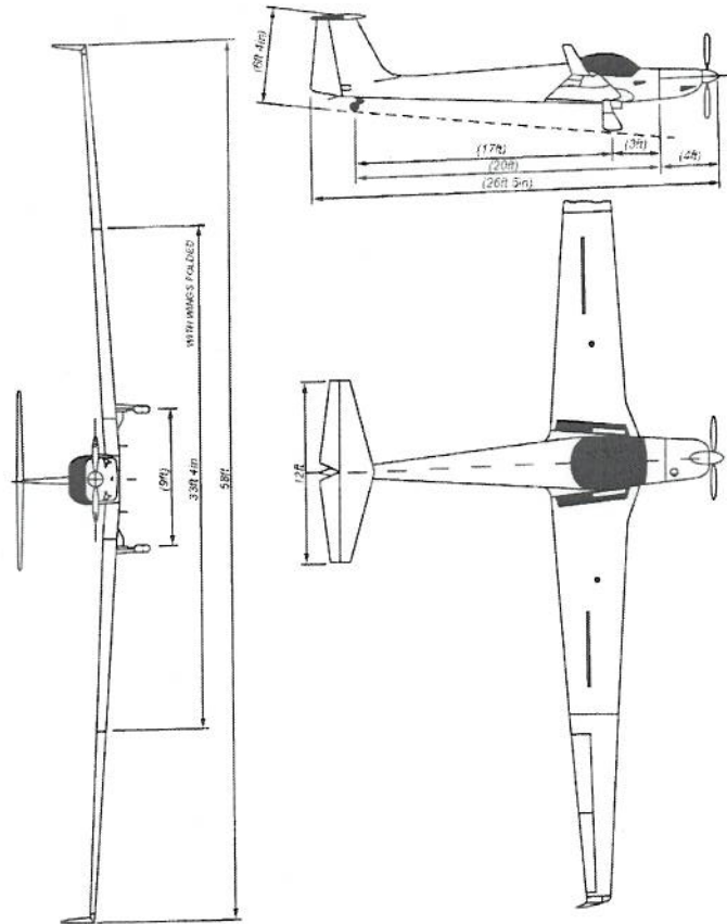
Figure 1. TG-14A Dimensions
