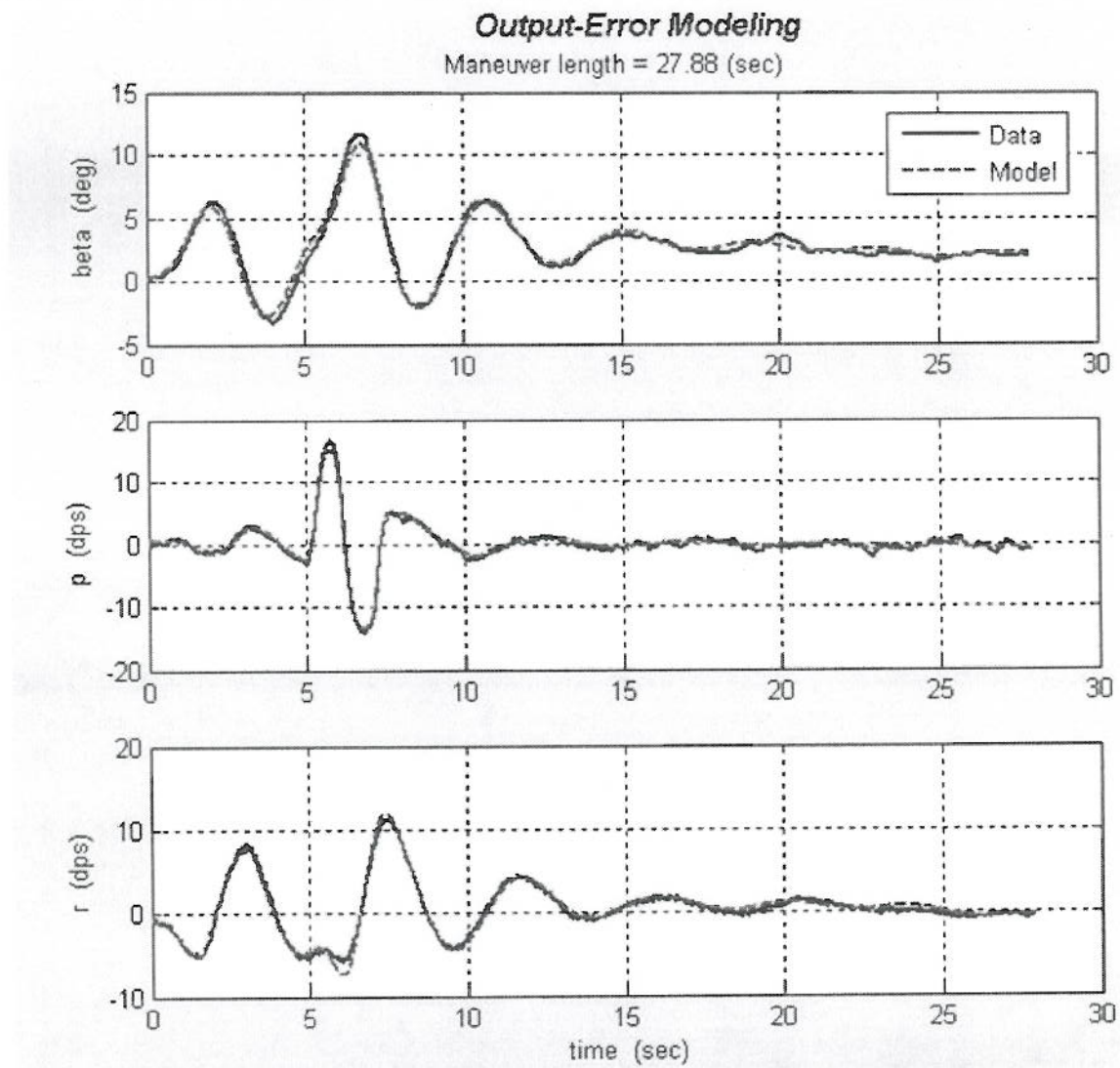
Figure E-3: Sample Results from a Yaw Roll Doublet (Wingtips On, Glide, 60 KIAS)
