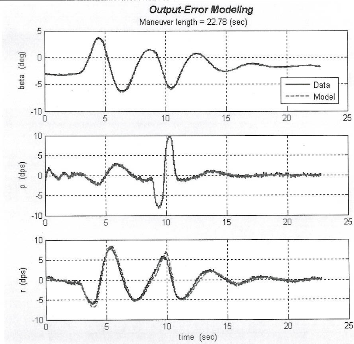
Figure E-8: Sample Results from a Yaw Roll Doublet (Wingtips Off, Glide, 60 KIAS)
