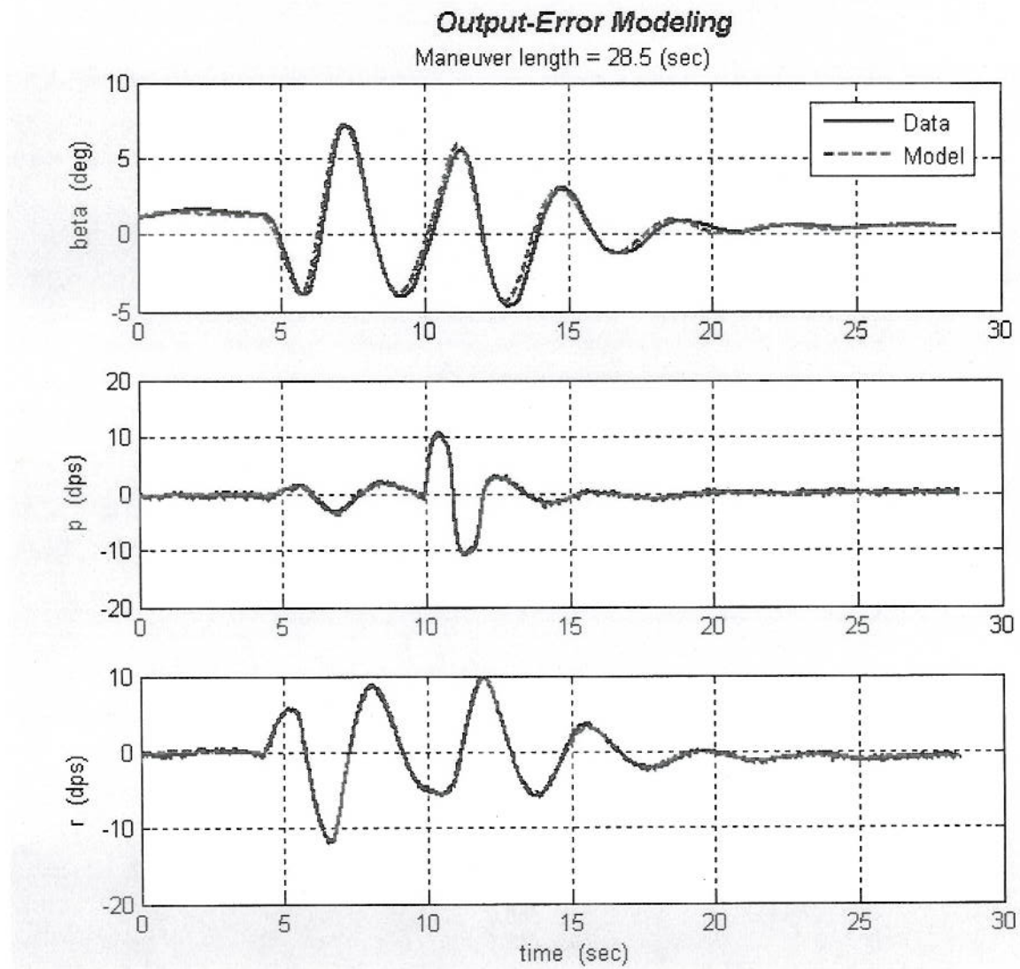
Figure E-12: Sample Results from a Yaw Roll Doublet (Wingtips Off, Power On, 60 KIAS)
