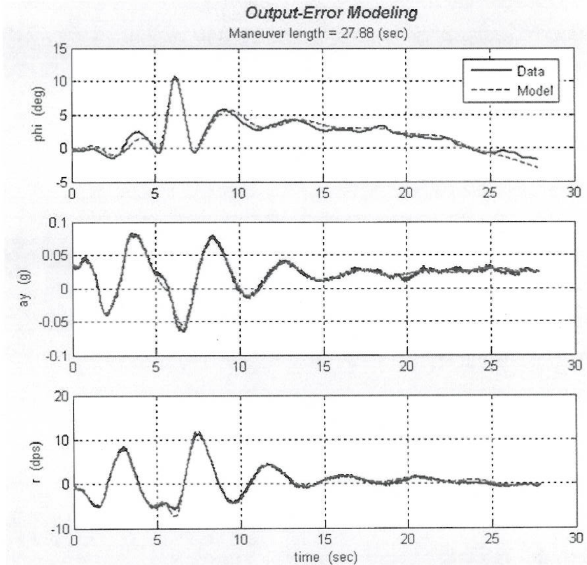
Figure E-2: Sample Results from a Yaw Roll Doublet (Wingtips On, Glide, 60 KIAS)
