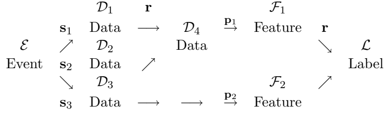
Figure 2.2: Label Fusion After Data Fusion Has Occurred.
