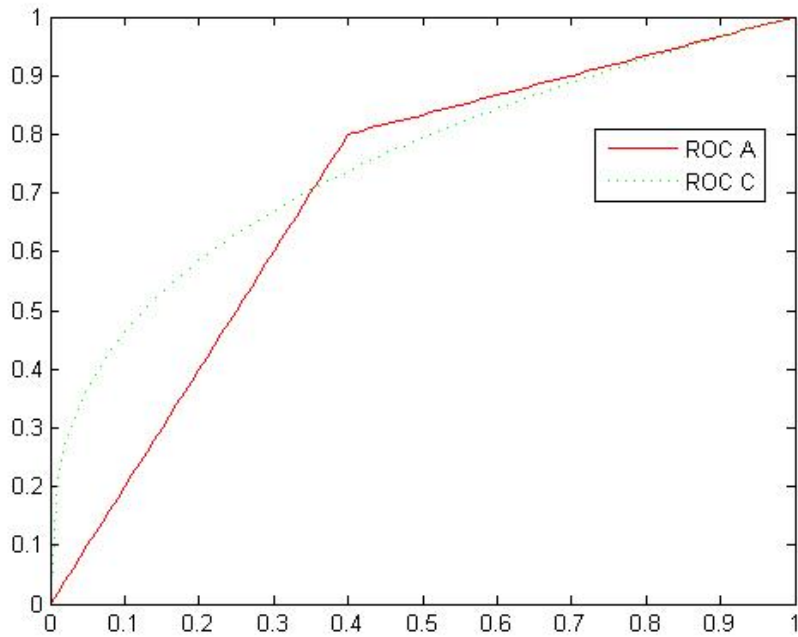
Figure 4.1: ROC Curves of Classification System Families \mathbb{A} and \mathbb{C} .
