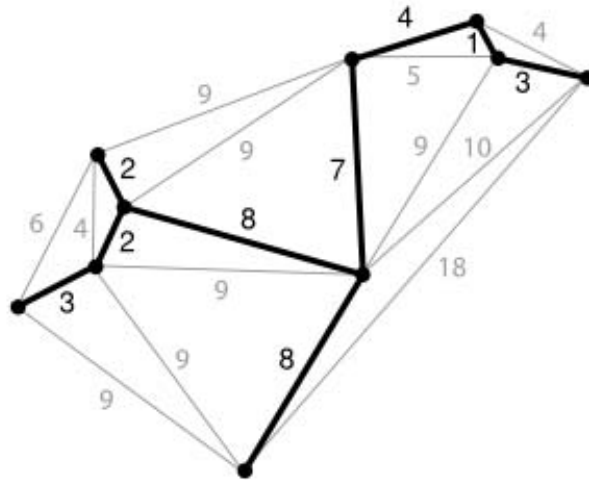
Figure 7. Example of a minimum spanning tree.
