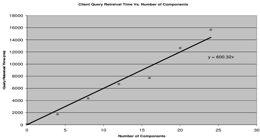
Figure 5.9 (a) Variation of CQRRT V Number of Components, .NET URDS
